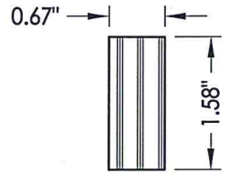
3C STILE LVL Reinforcement
