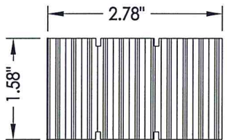
3E STILE LVL Reinforcement
