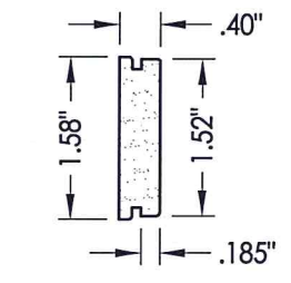
3B STILE Cellular PVC
