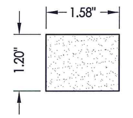
3A TOP RAIL Cellular PVC
