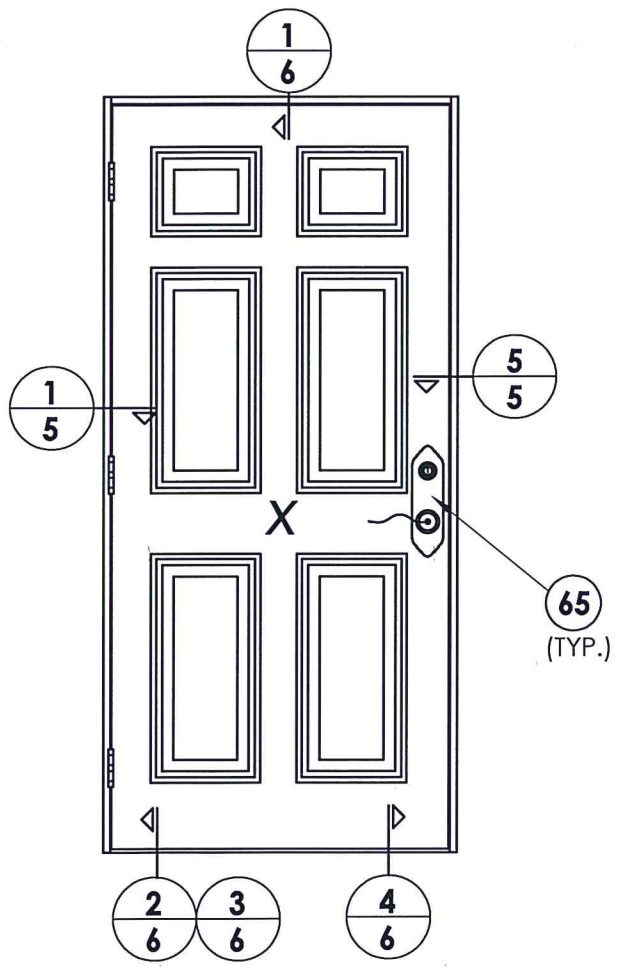
ELEVATION (X)
