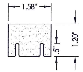
3D BOTTOM RAIL Cellular PVC
