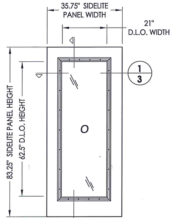
50 SIDELITE PANEL
