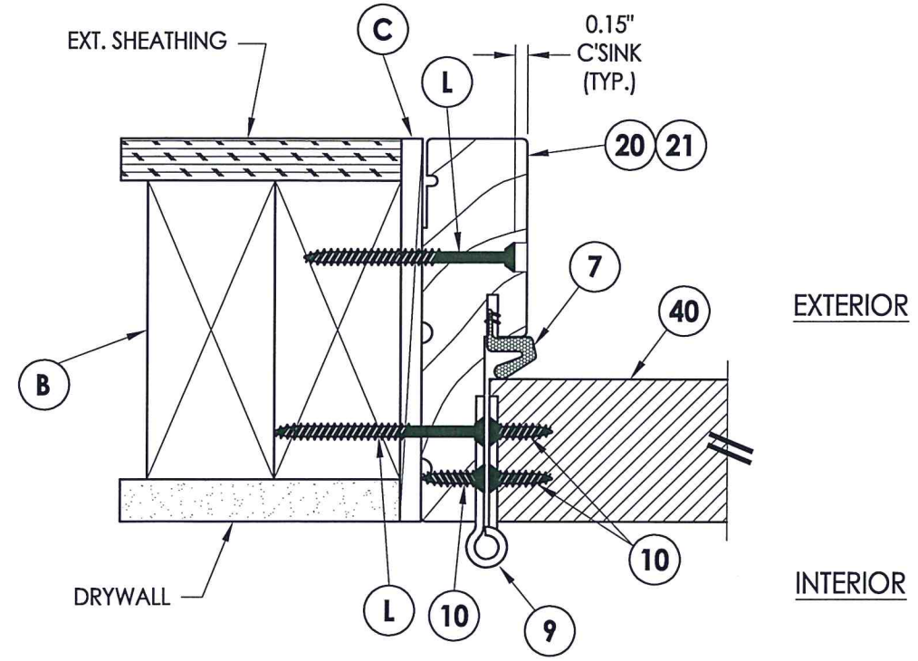
1 HORIZONTAL CROSS SECTION 5 Inswing shown - outswing also approved
