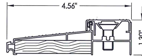
70 INSWING THRESHOLD
