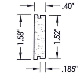
3B STILE Cellular PVC
