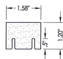
3D BOTTOM RAIL Cellular PVC
