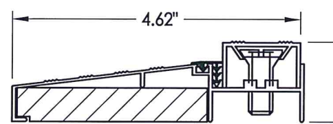
73 SIDELITE THRESHOLD
