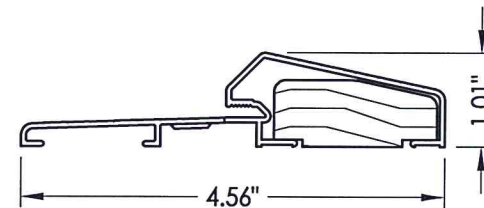
72 OUTSWING THRESHOLD
