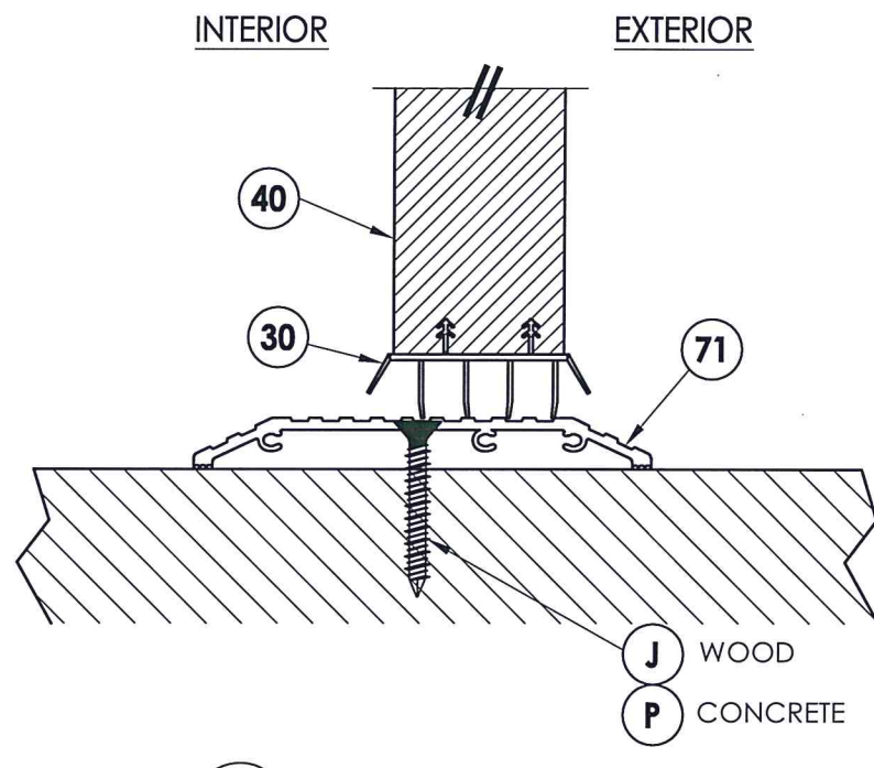
3 VERTICAL CROSS SECTION 6 Shown w/ ADA threshold
