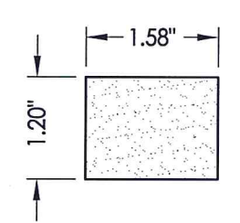
3A TOP RAIL Cellular PVC
