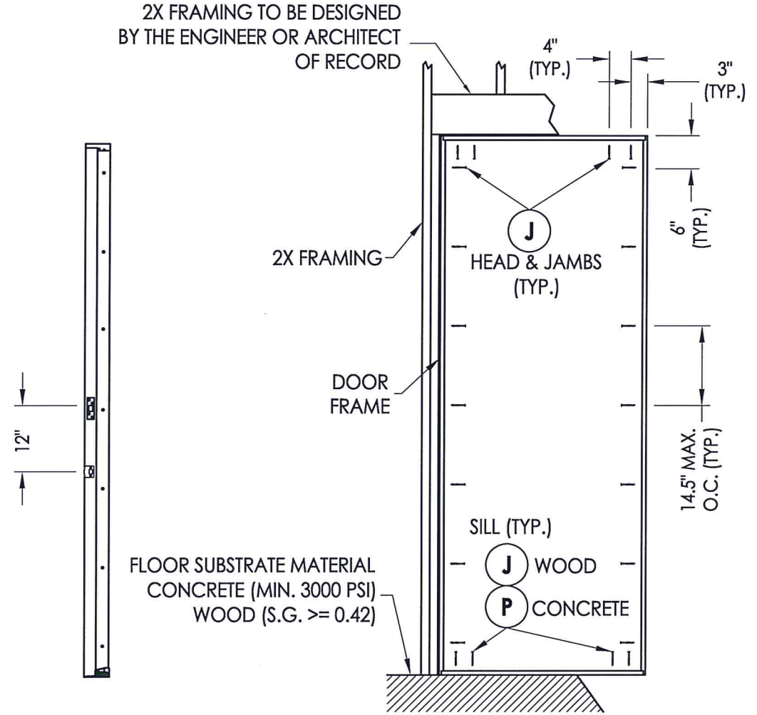
FRAME ANCHORING Stud construction
