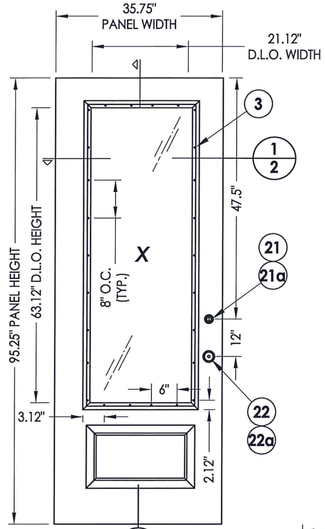
40 DOOR PANEL Fiberglass
