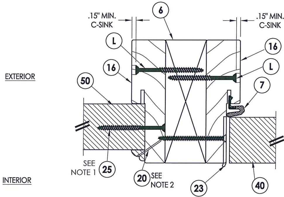
2 5 HORIZONTAL CROSS SECTION
