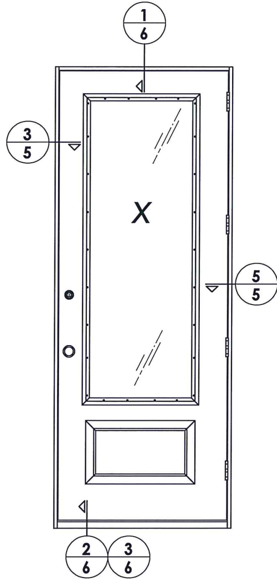
ELEVATION (X)
