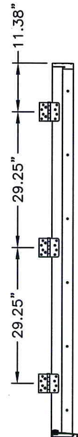
HINGE LOCATIONS
