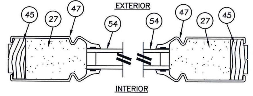
1 HORIZONTAL CROSS SECTION 6 (CLASSIC CRAFT)
