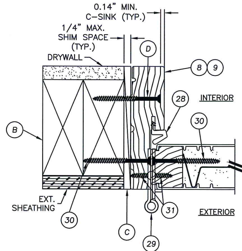
1 HORIZONTAL CROSS SECTION 7 OUTSWING SHOWN - INSWING ALSO APPROVED SMOOTH STAR PANEL SHOWN SEE DOOR PANEL DETAILS FOR OPTIONAL PANEL TYPES
