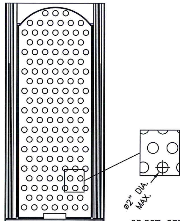
28.86% OPEN AREA MAX.
