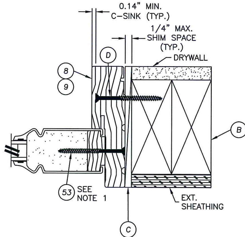
3 HORIZONTAL CROSS SECTION 7 OUTSWING SHOWN - INSWING ALSO APPROVED SMOOTH STAR PANEL SHOWN SEE DOOR PANEL DETAILS FOR OPTIONAL PANEL TYPES
