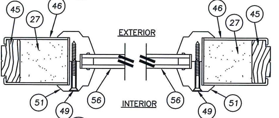
3 HORIZONTAL CROSS SECTION 6 (SMOOTH STAR)
