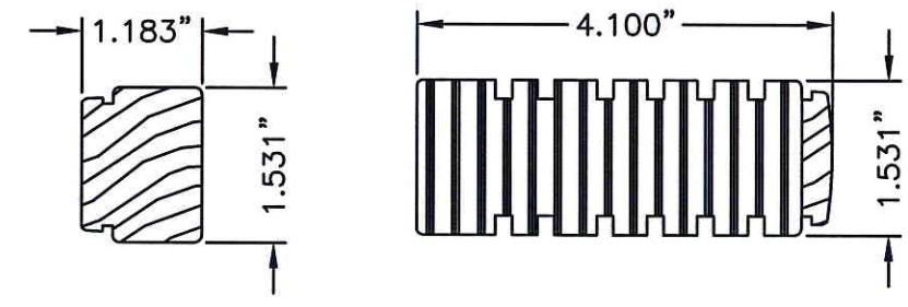
10 HINGE STILE SMOOTH STAR 11 LOCK STILE SMOOTH STAR
