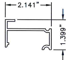
41 IN SWING SIDELITE SPACER
