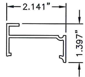
40 IN SWING SIDELITE SPACER
