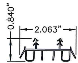
52 SWEEP
