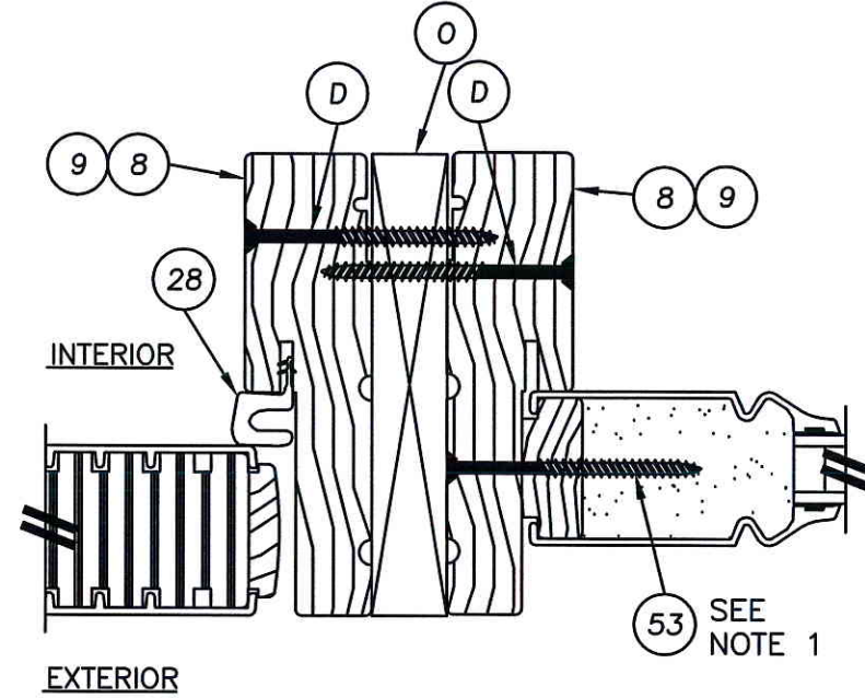
2 HORIZONTAL CROSS SECTION 7 OUTSWING SHOWN - INSWING ALSO APPROVED SMOOTH STAR PANEL SHOWN SEE DOOR PANEL DETAILS FOR OPTIONAL PANEL TYPES
