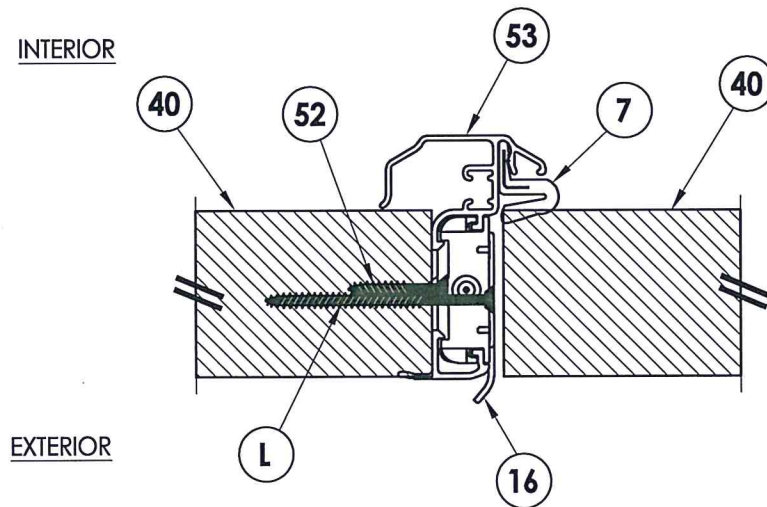
3 HORIZONTAL CROSS SECTION 6 Outswing shown - Inswing also approved
