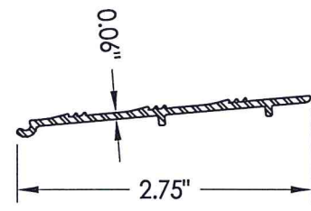
42 SILL EXTENDER
