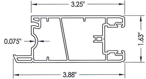
8 PD SASH Jamb Stile
