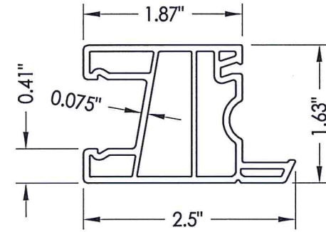
7 PD SASH Meeting Stile
