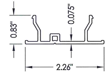
11 JAMB COVER
