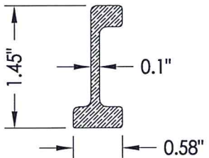
12 REINFORCEMENT Meeting Stiles
