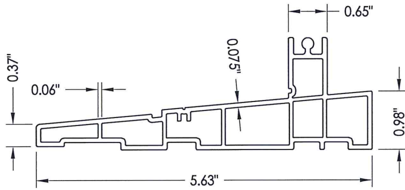
5 PD SILL
