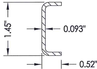
13 REINFORCEMENT Lock Stile
