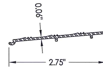
42 SILL EXTENDER
