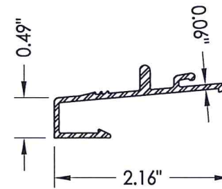
41 SILL NOSING
