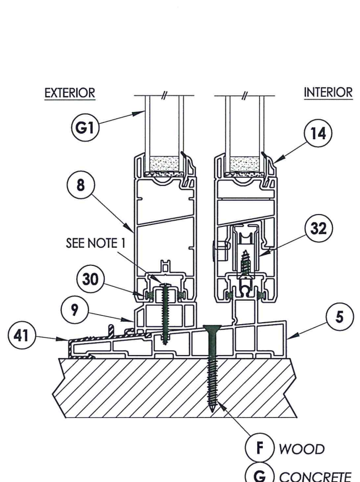
3 2 VERTICAL CROSS SECTION
