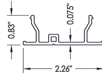
11 JAMB COVER
