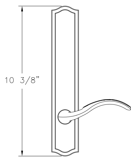
PASSIVE DOOR HANDLE SET DIE CAST
