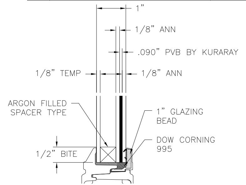
GLAZING DETAIL
