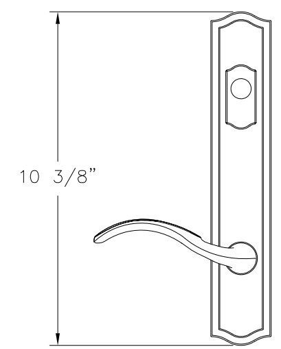
ACTIVE DOOR HANDLE SET DIE CAST
