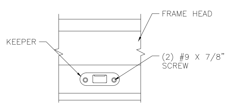
HEAD BAR KEEPER DETAIL
