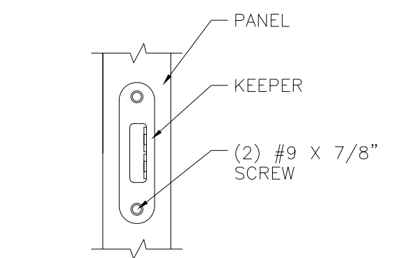
HOOK KEEPER DETAIL
