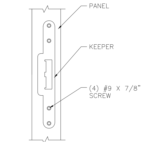
SLAB MULTI-POINT LOCK KEEPER DETAIL
