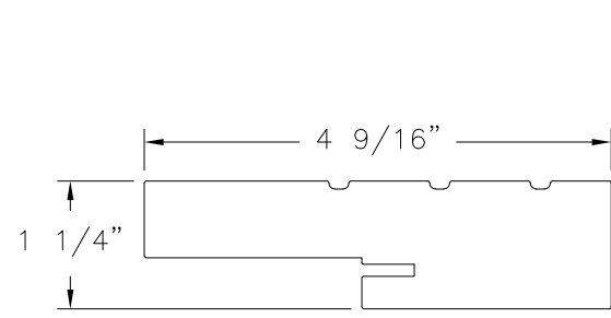
HEAD FRAME & JAMB FOAM PVC CO-EX
