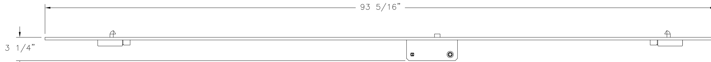
MULTI-POINT LOCKING SYSTEM STAINLESS STEEL (SS930) BY JAM YUAN ENTERPRISES CO., LTD.
