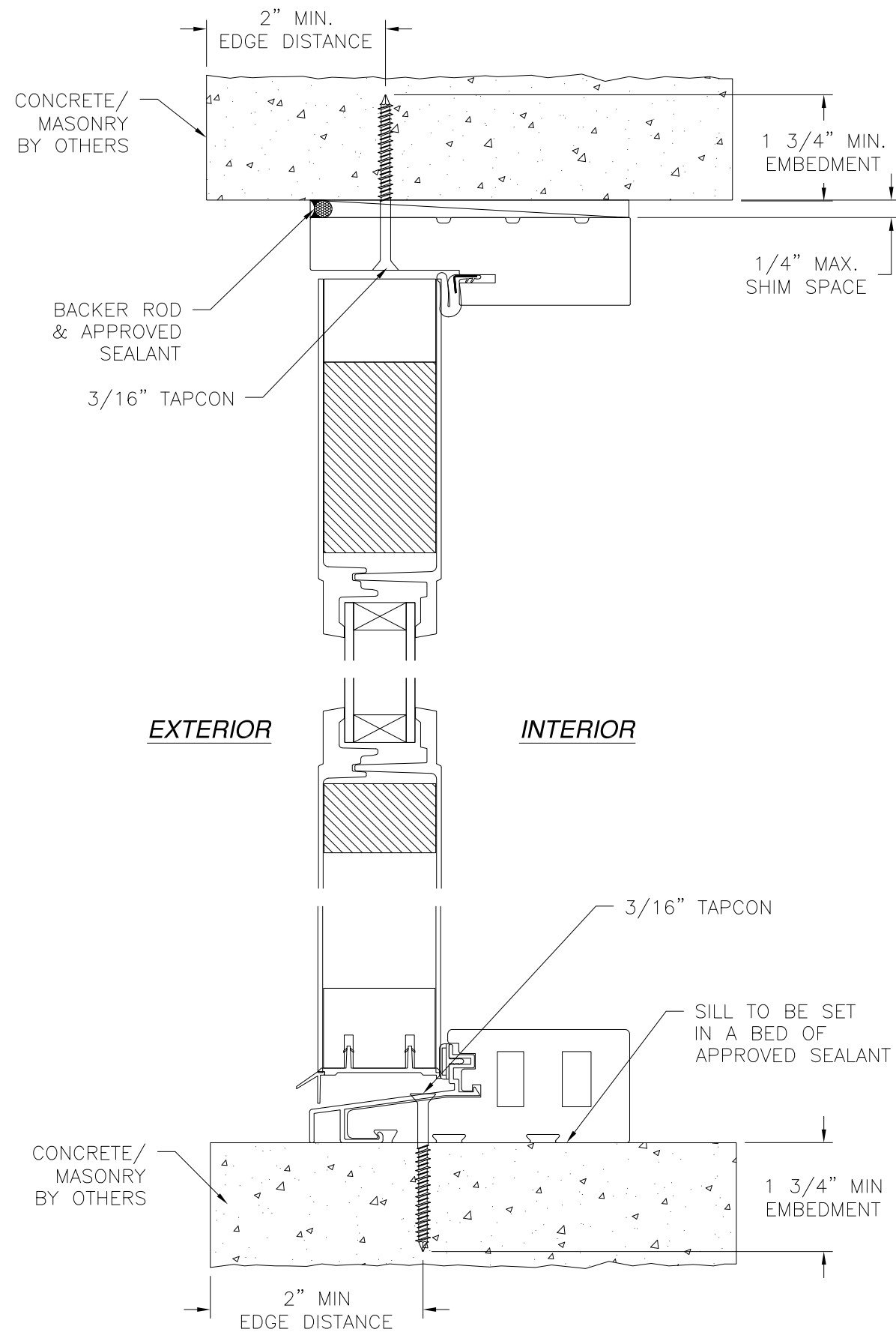
DOOR INSTALLATION DETAIL CONCRETE/MASONRY INSTALLATION
