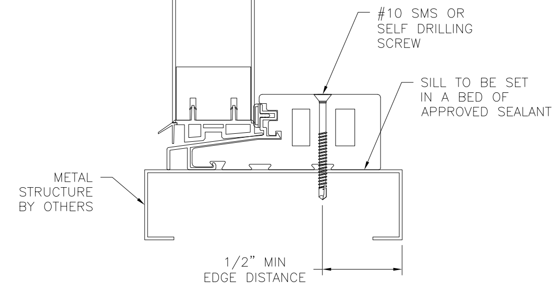
SIDELITE DOOR INSTALLATION DETAIL METAL STRUCTURE INSTALLATION
