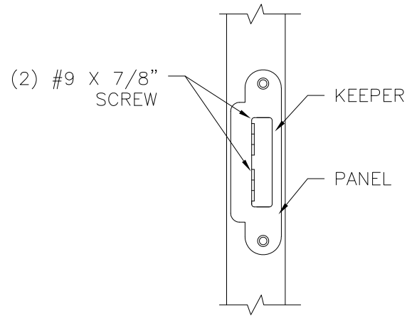
SLAB MULTI-POINT LOCK KEEPER DETAIL
