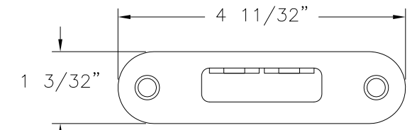
HOOK KEEPER STAINLESS STEEL (SS92G) BY JAM YUAN ENTERPRISES CO., LTD
