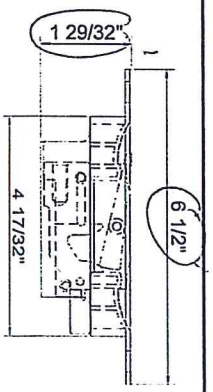
29 FLUSH BOLT MECHANISM DIE CAST, STEEL, POM
