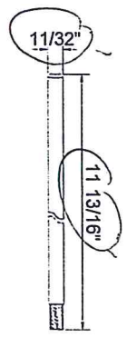
28 FLUSH BOLT BAR STAINLESS STEEL
