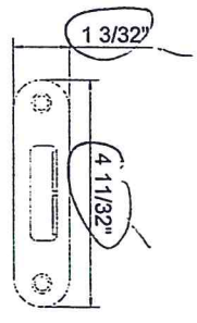
32 HEAVY HOOK KEEPER STAINLESS STEEL
