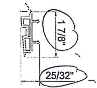
13 DOOR BOTTOM-(B) RIGID PVC CO-EX
