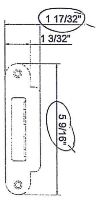
34 SLAB MULTI-POINT LOCK KEEPER STAINLESS STEEL
