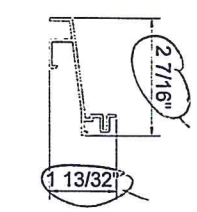
11 OUTSWING SILL-(B) ALUMINIUM
