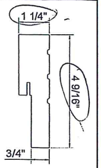
1 HEAD FRAME & JAMB FOAM PVC CO-EX.
