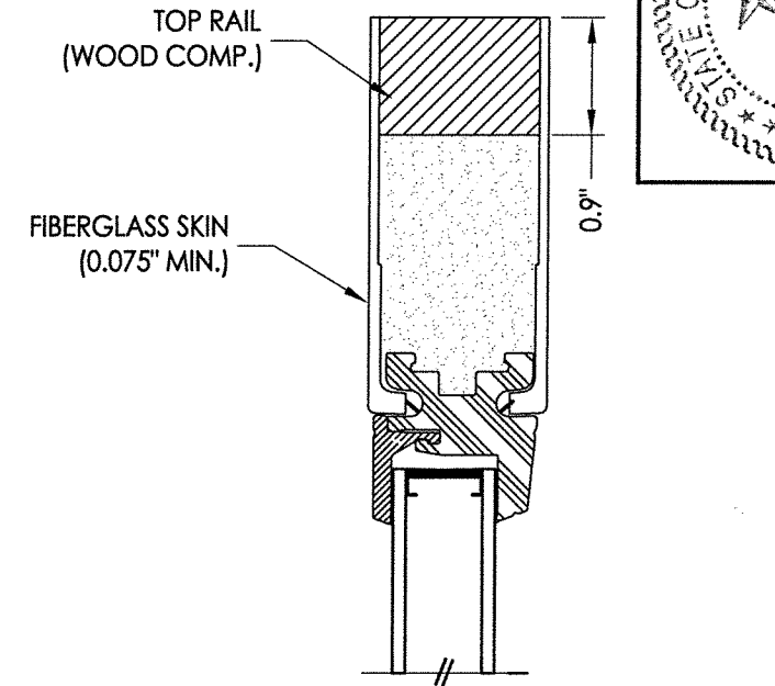
2 3 VERTICAL CROSS SECTION
