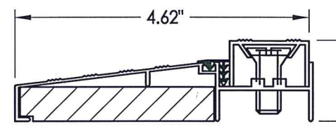
73 SIDELITE THRESHOLD
