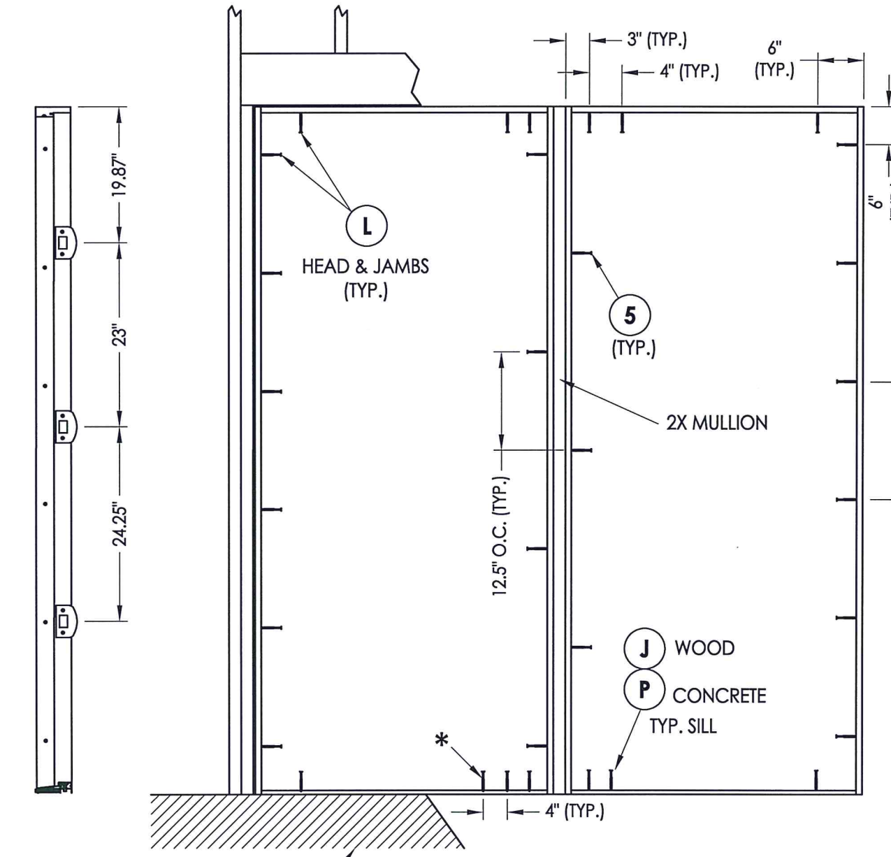
FRAME ANCHORING XO / OX
