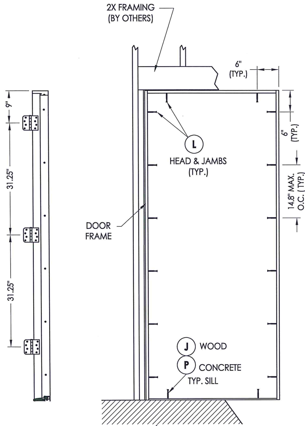
FRAME ANCHORING X
