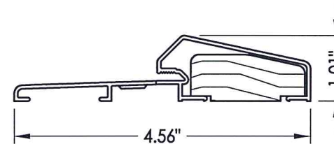
72 OUTSWING THRESHOLD
