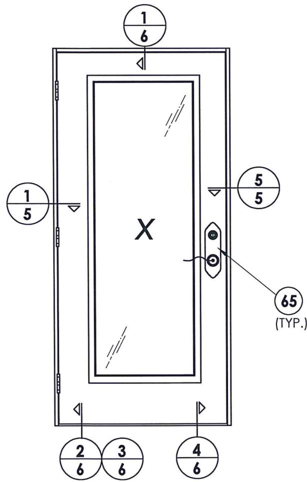
ELEVATION (X)
