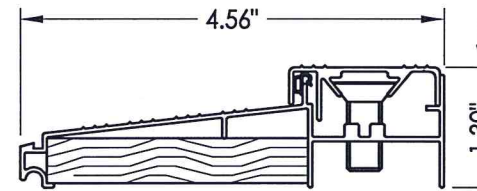
70 INSWING THRESHOLD
