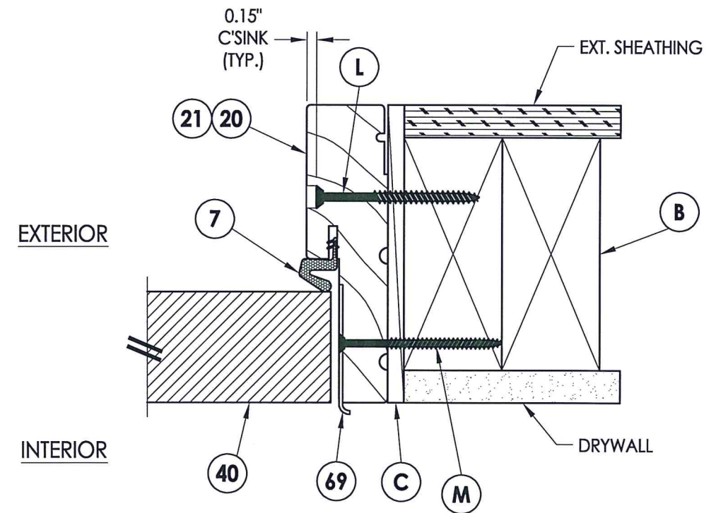
5 5 HORIZONTAL CROSS SECTION Inswing shown - outswing also approved
