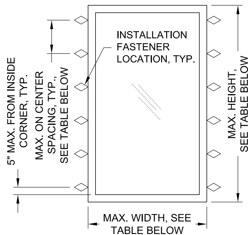
REPLACEMENT ELEVATION SEE DETAILS SHEET 2
