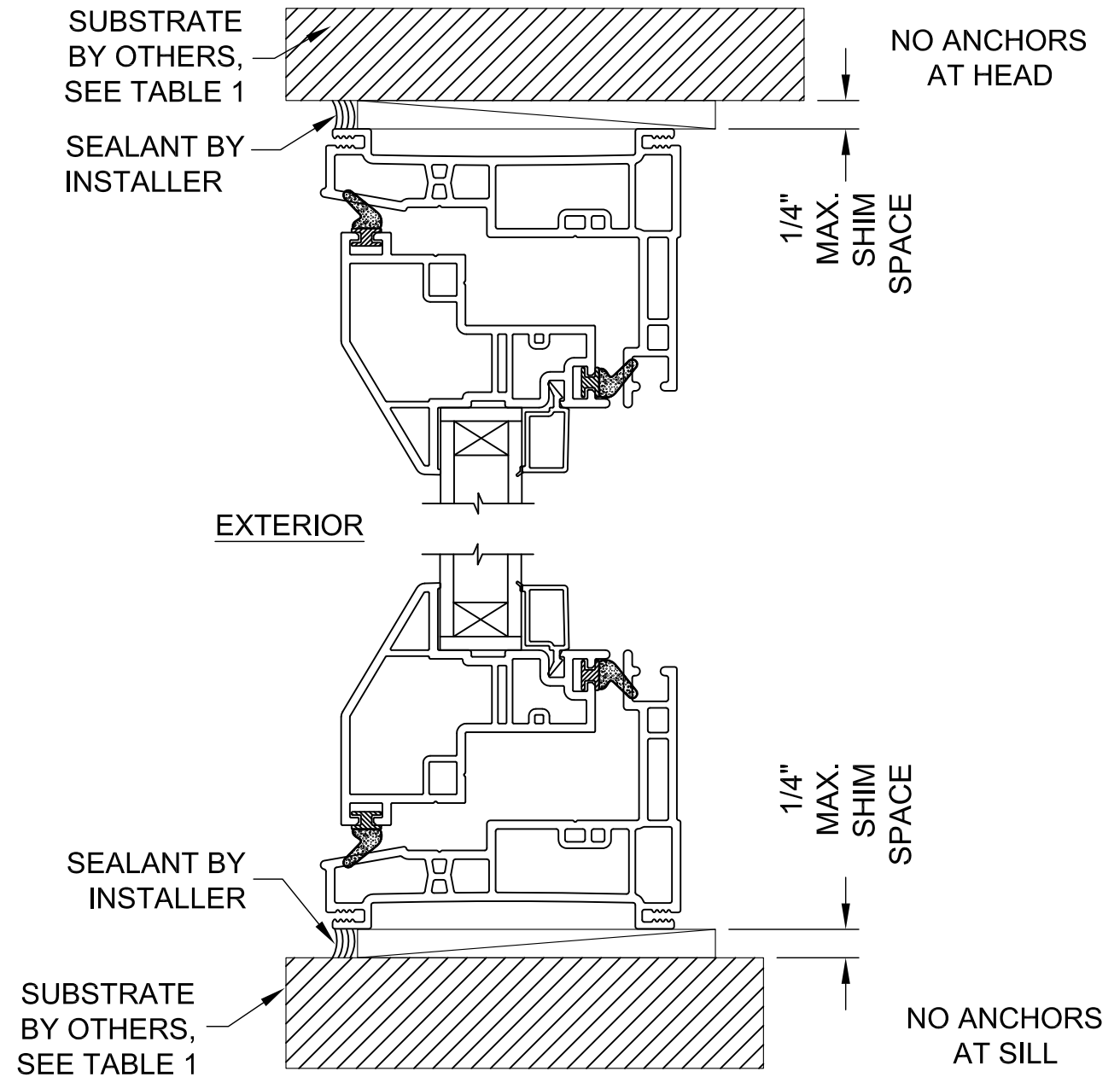
TYPICAL FRAME VERTICAL SECTION
