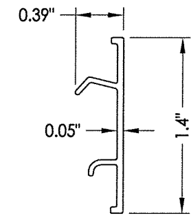
12 FRAME ADAPTER
