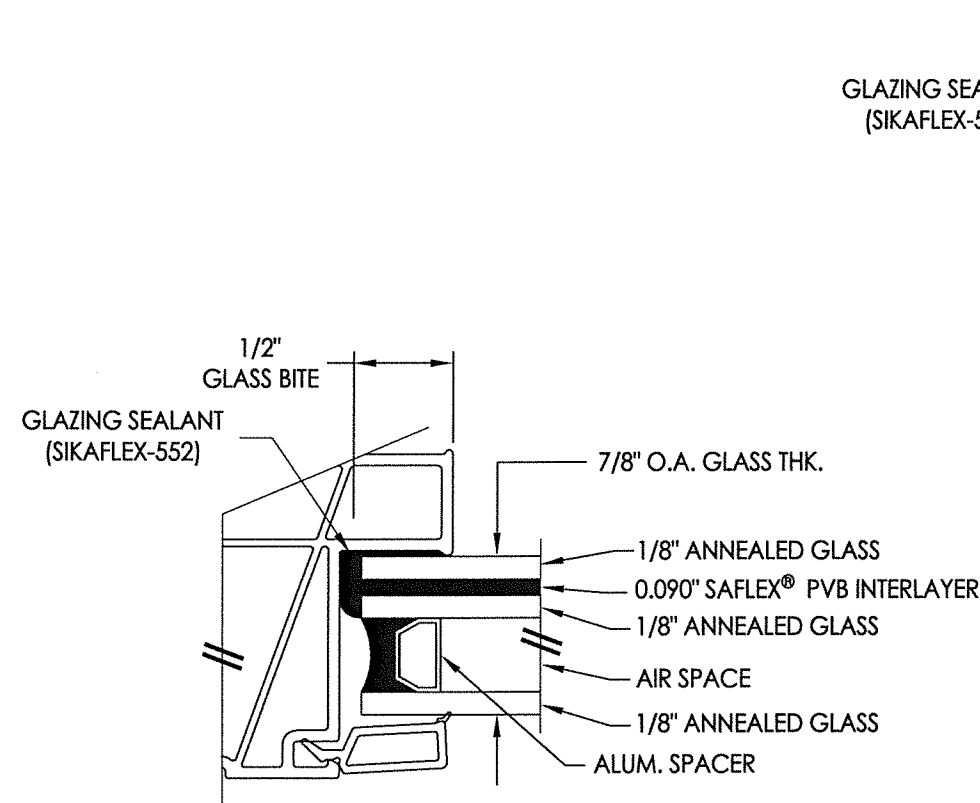
G1 GLAZING DETAIL
