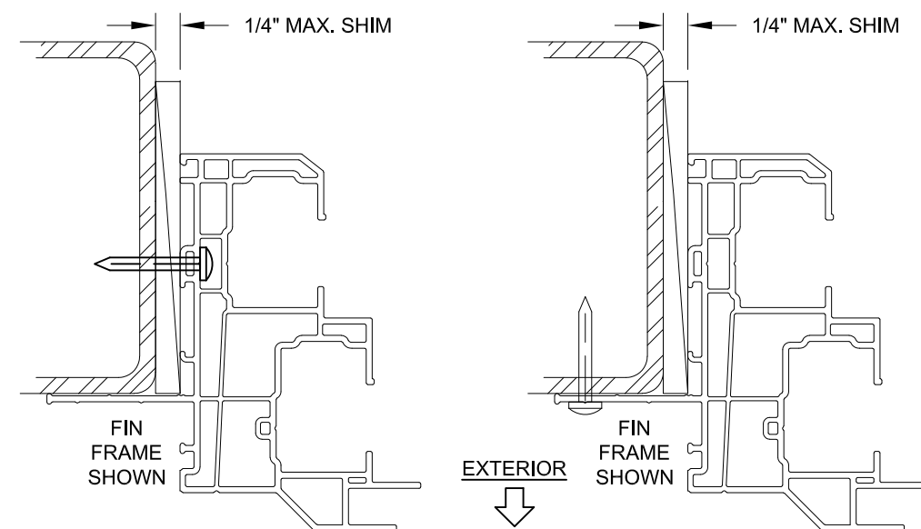
INSTALLATION THROUGH THE FRAME, INTO METAL
