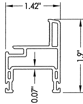
6 SLIDER COMMON RAIL
