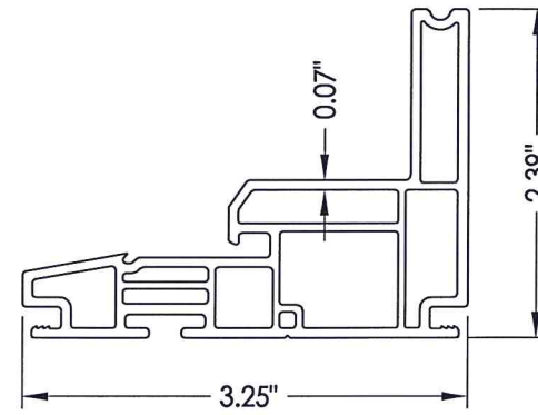
1 FRAME
