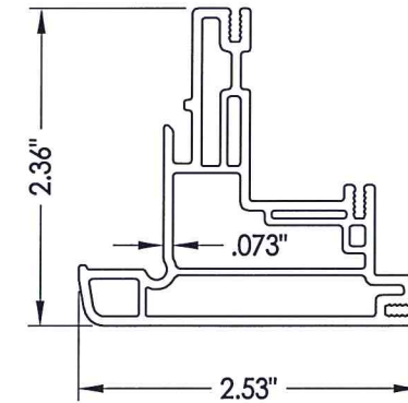
2 SASH
