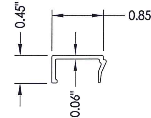
3 GLAZING BEAD
