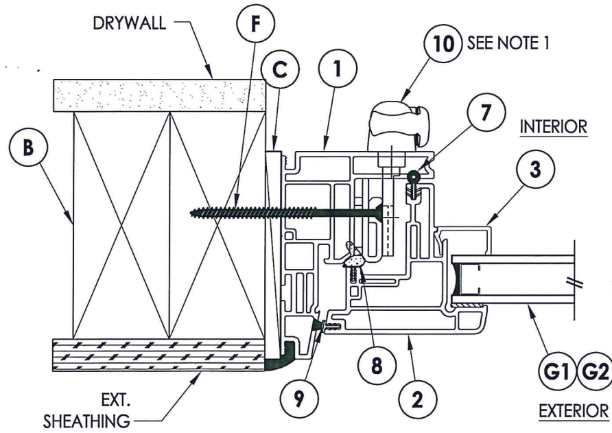
1 2 HORIZONTAL CROSS SECTION
