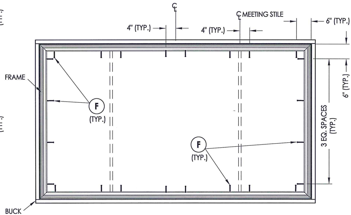
FRAME ANCHORING 1/4 - 1/2 - 1/4
