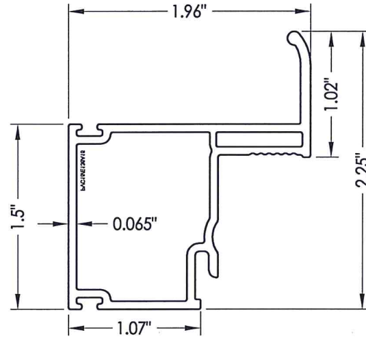
5 HANDLE SASH
