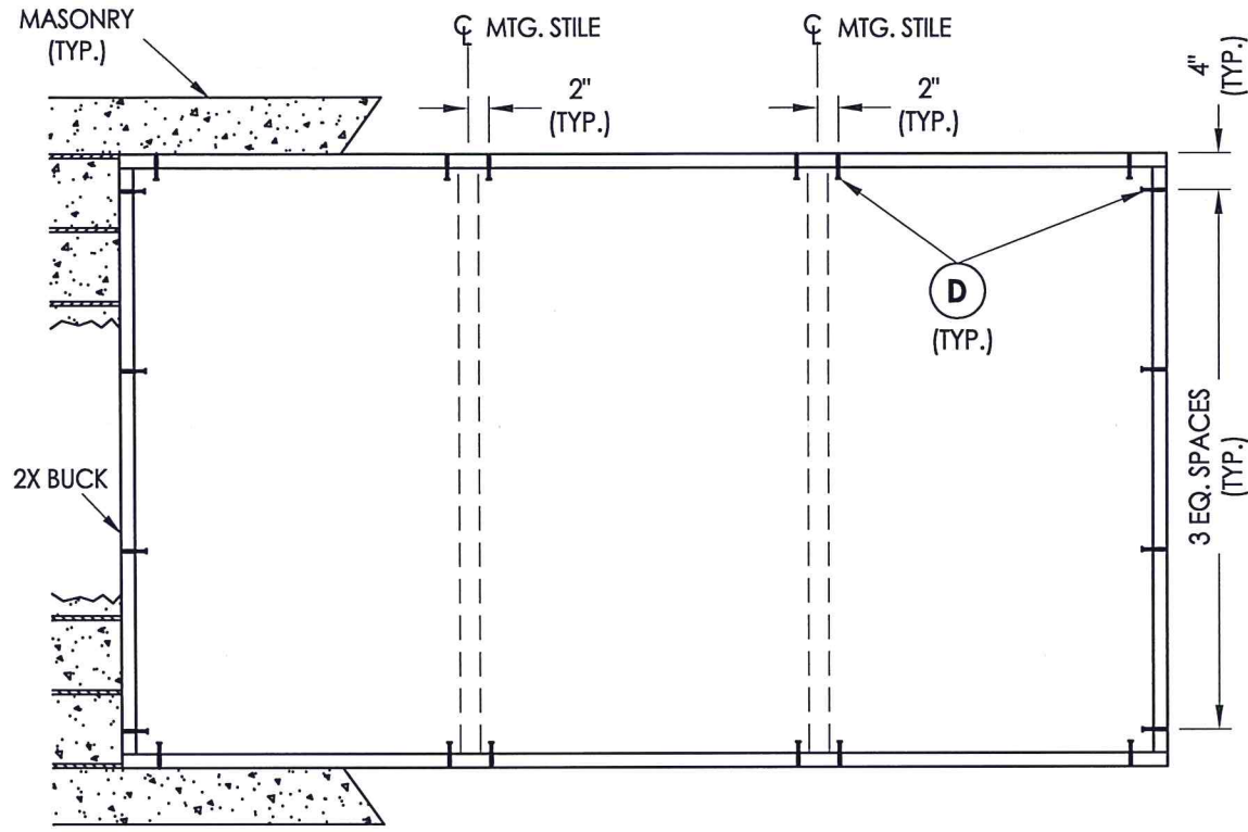
BUCK ANCHORING 1/3 - 1/3 - 1/3
