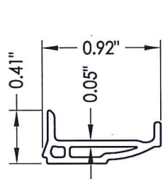
9 GLAZING BEAD
