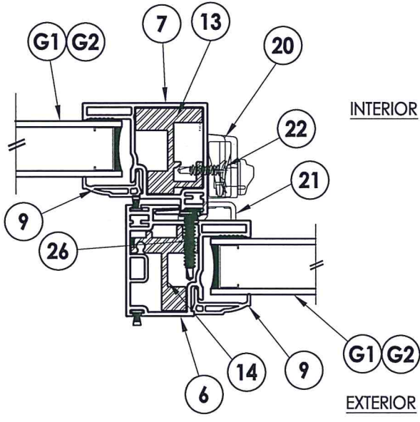
1 HORIZONTAL CROSS SECTION 2X Buck Construction
