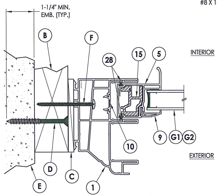
1 HORIZONTAL CROSS SECTION 2X Buck Construction
