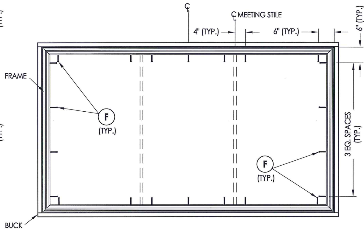
FRAME ANCHORING 1/3 - 1/3 - 1/3
