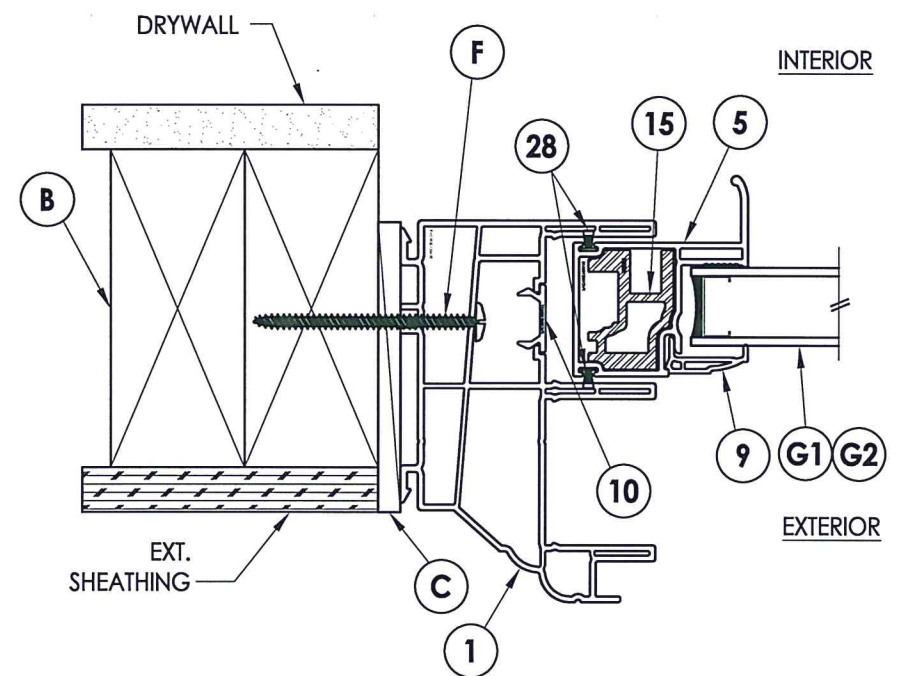
2 HORIZONTAL CROSS SECTION Shown w/ Stud Framing
