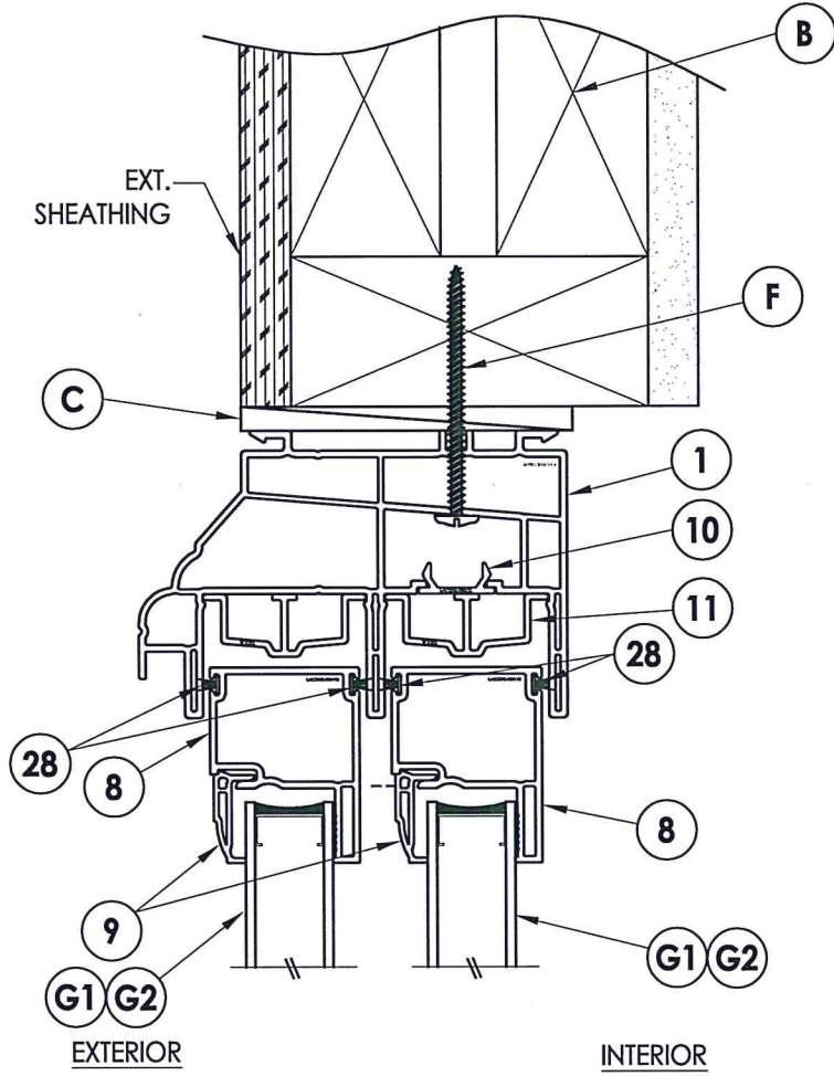
1 VERTICAL CROSS SECTION 3 Shown w/ Stud Framing
