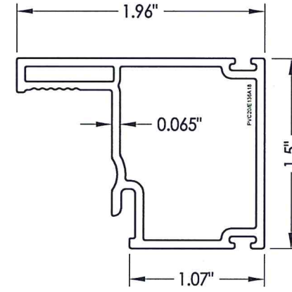
8 MAIN SASH
