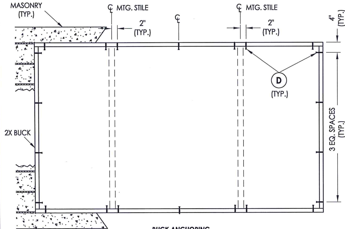
BUCK ANCHORING 1/4 - 1/2 - 1/4
