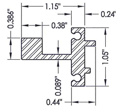
14 REINFORCEMENT
