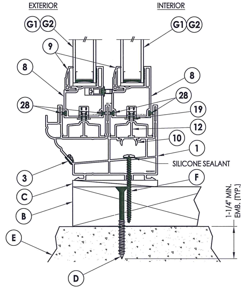
2 VERTICAL CROSS SECTION 3 2X Buck Construction
