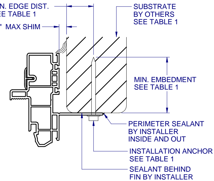
D HORIZONTAL SECTION 6 BOX FRAME INSTALLATION HEAD AND SILL SIMILAR FOR BOX INSTALLATION
