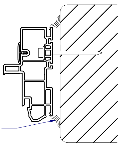
B HORIZONTAL SECTION 6 TYPICAL JAMB ANCHORAGE
