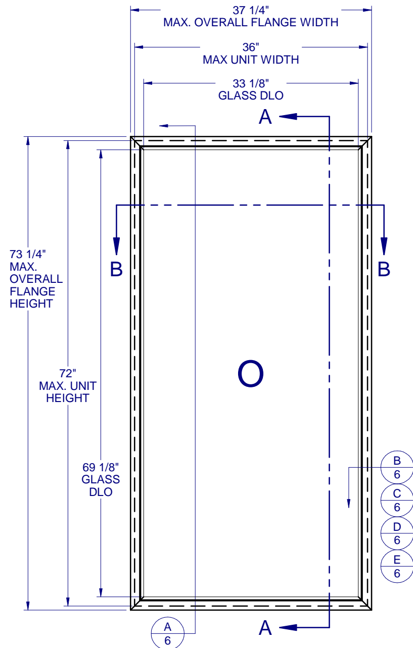
SYSTEM 1 & 2 (CAR 138-535/138-1094/138-540/138-1318) MAXIMUM ALLOWABLE DESIGN PRESSURE: +55/-55 PSF
