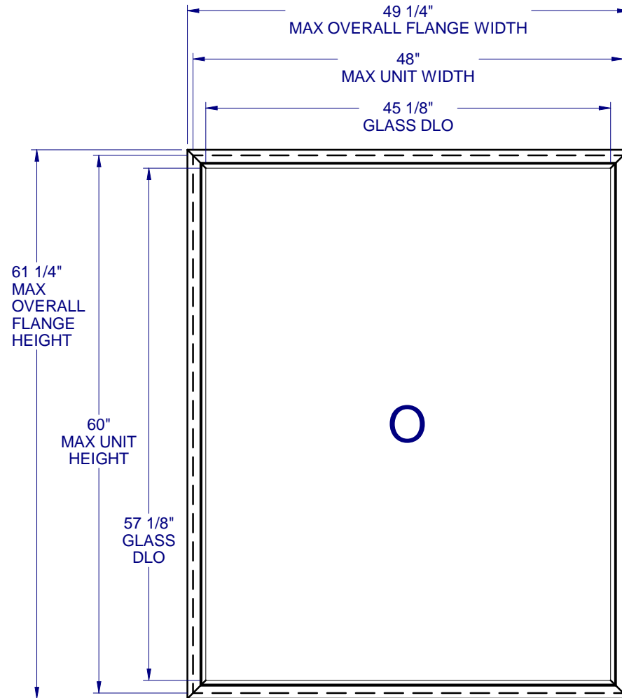
SYSTEM 3 (CAR 138-539/138-1317) MAXIMUM ALLOWABLE DESIGN PRESSURE: +50/-50 PSF
