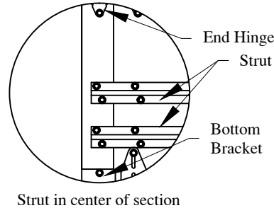
Detail E
