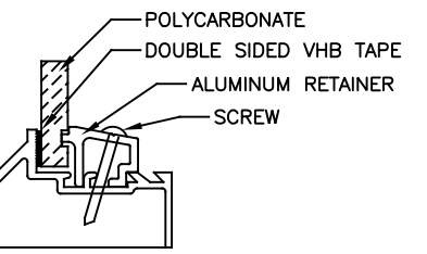
7 SECTION E-E POLYCARBONATE RETAINER
