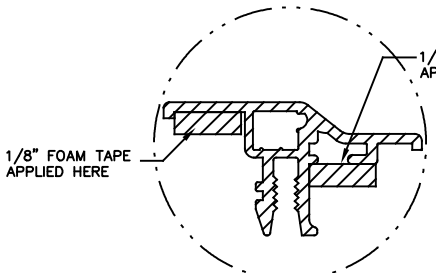
ALUMINUM FRAME (STATIC RATED ALTERNATE FRAME OPTION) DETAIL F
