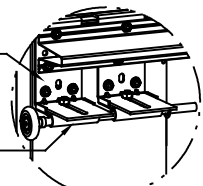
DETAIL A 1/8" BEAD OF BOSTICK 1100 OR EQUIVALENT
