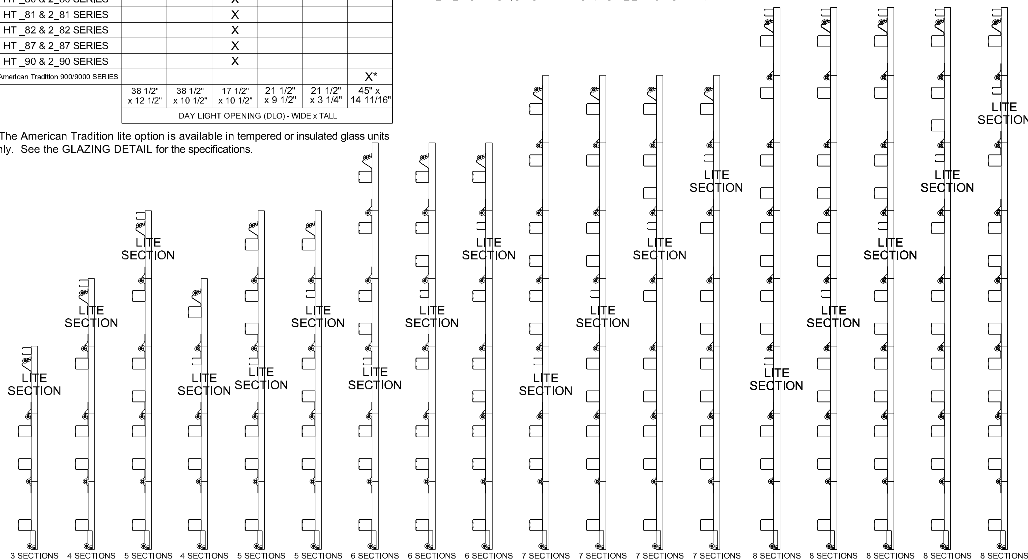
WITH LITE SECTION ANYWHERE EXCEPT THE TOP AND BOTTOM SECTION STRUT CONFIGURATION
