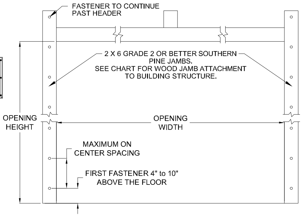
SCREW LOCATION - COMMERCIAL LITES NOTE: 10 SCREWS USED.
