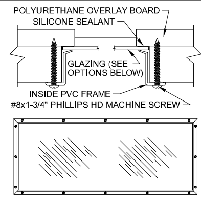
SCREW LOCATION - AM. TRADITION NOTE: 16 SCREWS USED.
