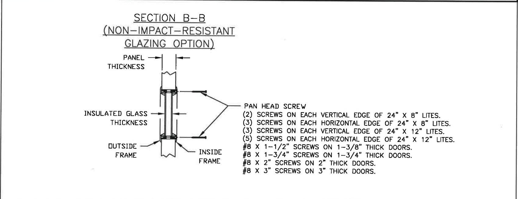
STANDARD ASSEMBLY DETAILS DRAWING 104039-B
