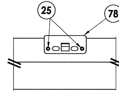
DETAIL 1 Multipoint Lock Strike Plate @ Head
