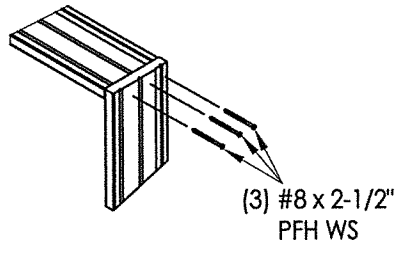
JAMB TO HEAD DETAIL (TYP.)
