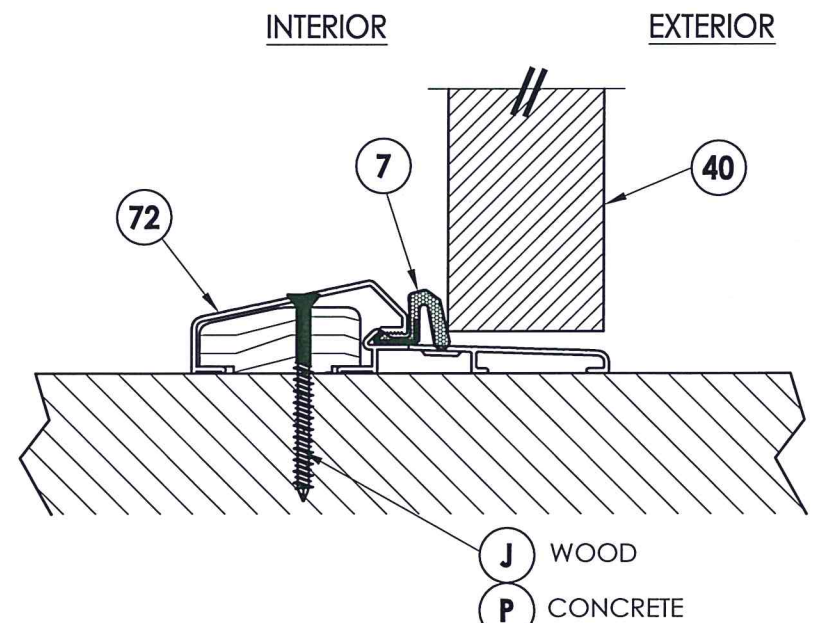
4 VERTICAL CROSS SECTION 6 Outswing configuration
