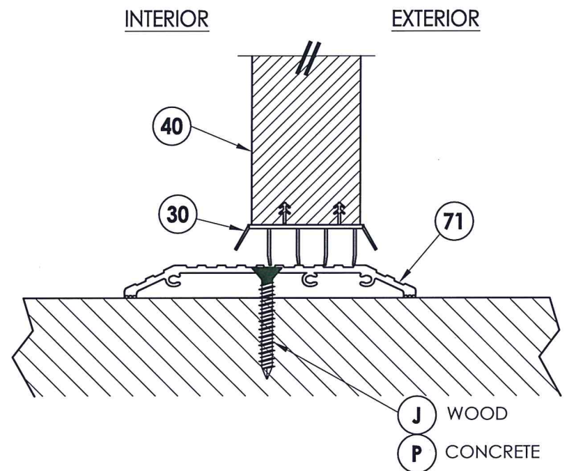
3 VERTICAL CROSS SECTION 6 Shown w/ ADA threshold
