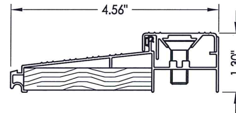
70 INSWING THRESHOLD
