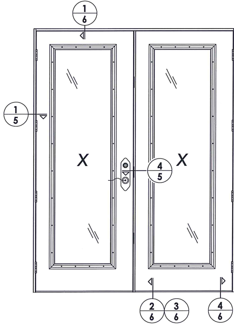
ELEVATION (XX)
