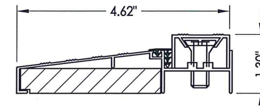
73 SIDELITE THRESHOLD
