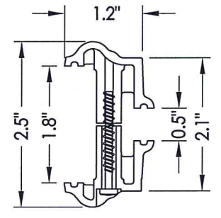
2F PLASTIC LIP LITE FRAME ODL
