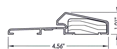
72 OUTSWING THRESHOLD
