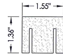
45 BOTTOM RAIL Composite
