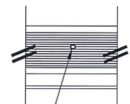
DETAIL 2 Astragal Strike Plate Outswing
