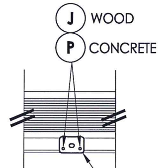
DETAIL 2 Astragal Strike Plate Inswing
