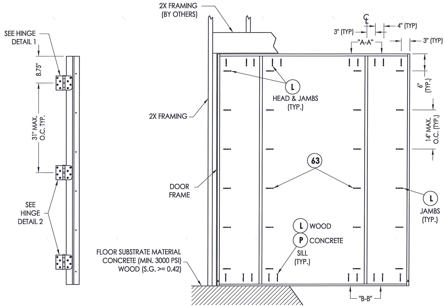
HINGE MULLION
