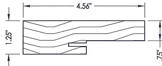
4 1 SIDE & HEAD JAMBS
