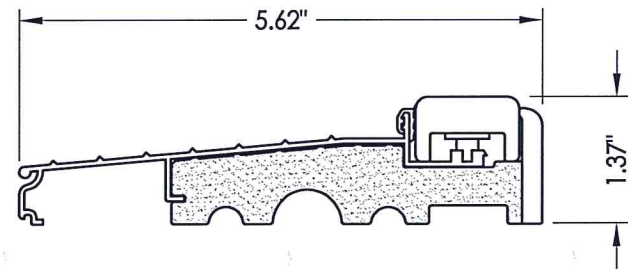
5 INSWING THRESHOLD
