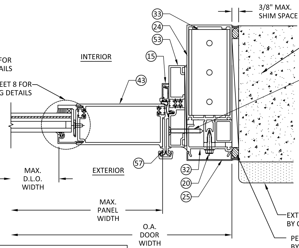
B HORIZONTAL SECTION 6 500T DOOR & 1600 WALL SYSTEM JAMB
