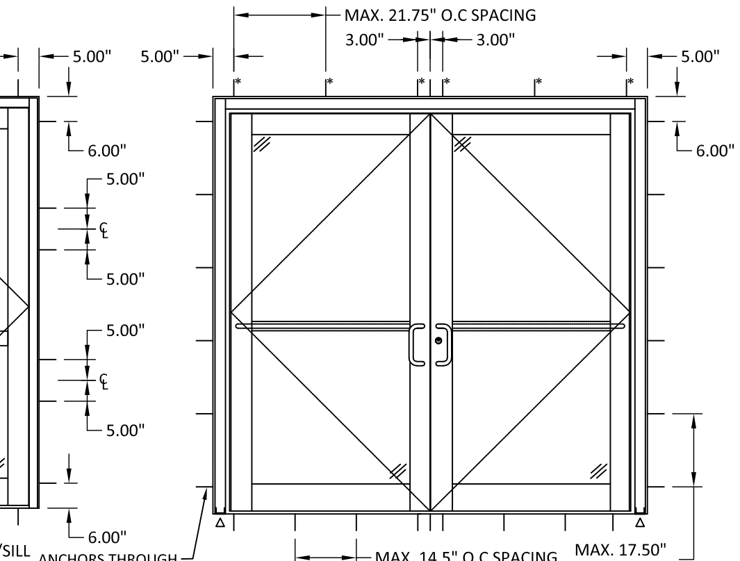
500T THERMAL DOOR WITH 1600 WALL SYSTEM
