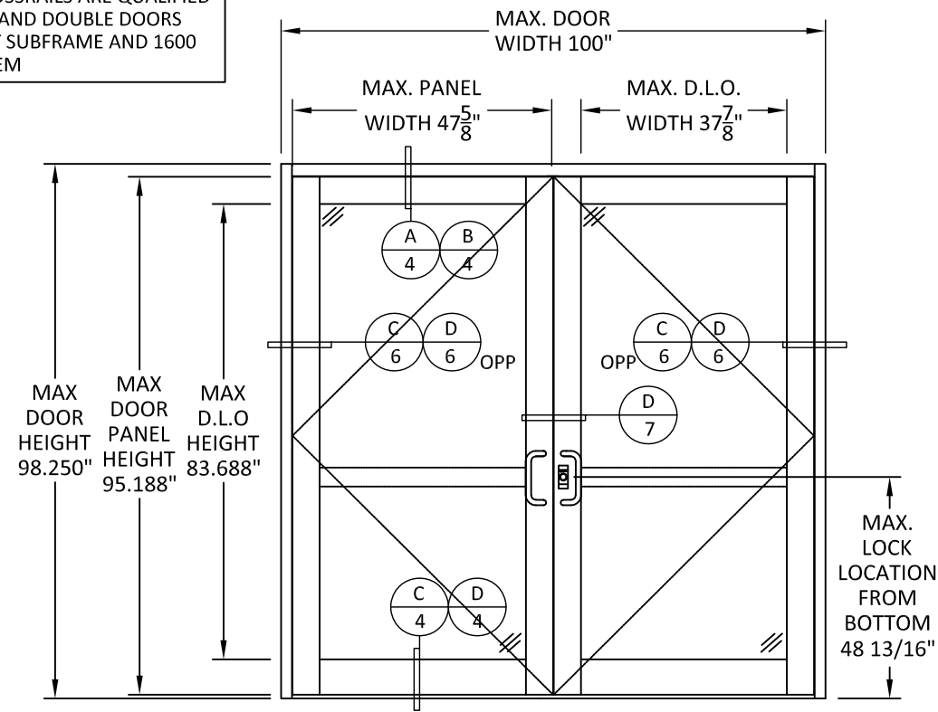
500T THERMAL DOOR WITH 451T SUBFRAME
