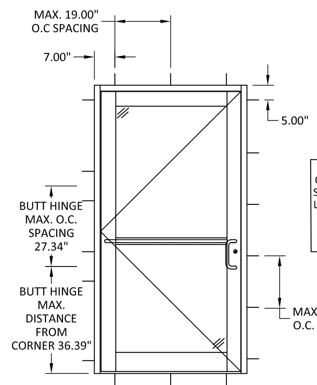
ANCHOR LAYOUT 500T THERMAL DOOR WITH 451T SUBFRAME W/ BUTT HINGE
