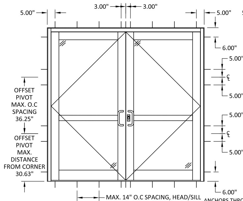
500T THERMAL DOOR WITH 451T SUBFRAME W/ OFFSET PIVOT
