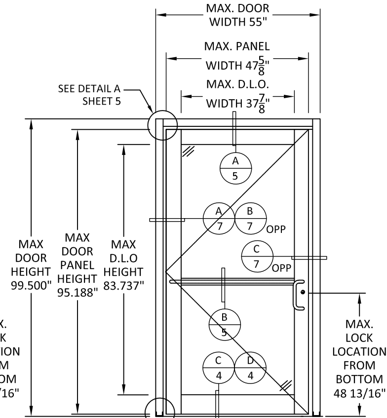
ELEVATION 500T THERMAL SINGLE DOOR WITH 1600 WALL SYSTEM
