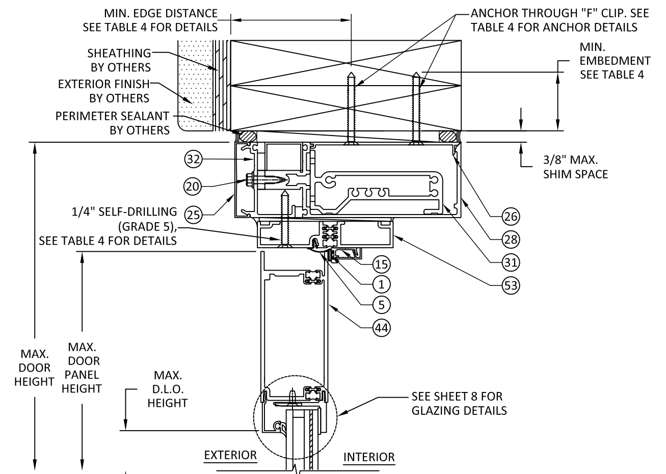
A 5 VERTICAL SECTION 500T DOOR & 1600 WALL SYSTEM SILL-2X WOOD FRAME
