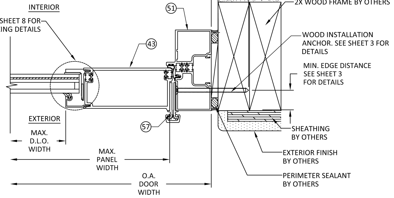
D HORIZONTAL SECTION 6 500T DOOR & TRIFAB 451T SUBFRAME JAMB-2X WOOD BUCK
