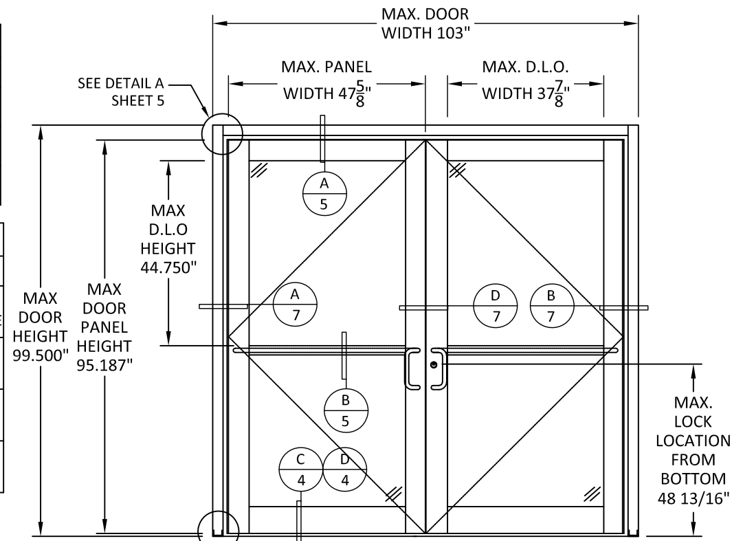
500T THERMAL DOOR WITH 1600 WALL SYSTEM
