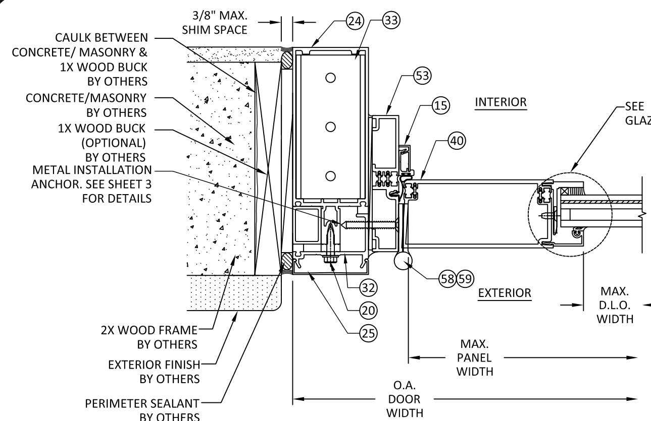
A HORIZONTAL SECTION 7 500T DOOR & 1600 WALL SYSTEM JAMB
