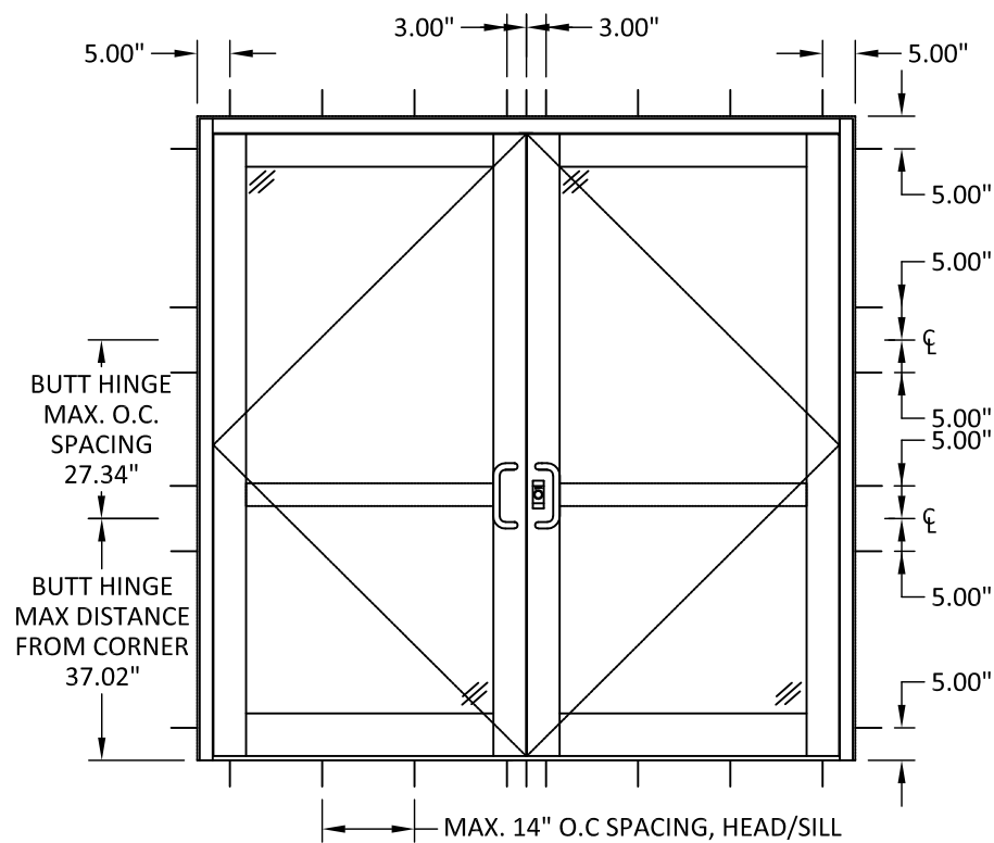
500T THERMAL DOOR WITH 451T SUBFRAME W/ BUTT HINGE
