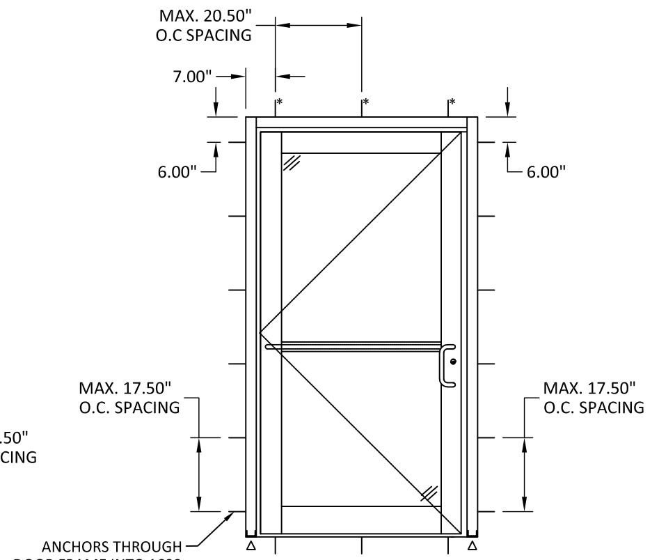
ANCHOR LAYOUT 500T THERMAL DOOR WITH 1600 WALLSYSTEM
