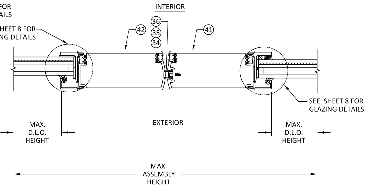
D HORIZONTAL SECTION 7 ASTRAGAL THERMALLY BROKEN
