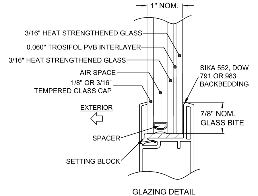
GLAZING DETAIL
