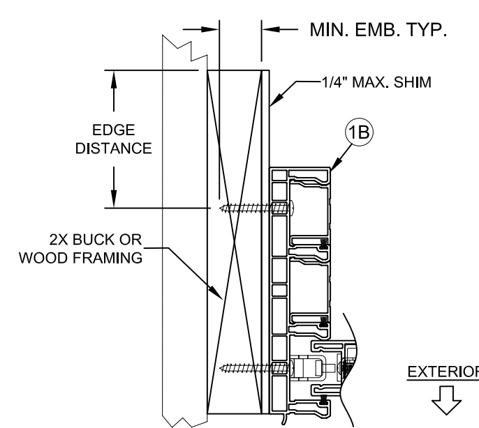
④ HORIZONTAL CROSS SECTION ③ 2X BUCK CONSTRUCTION (SEE NOTES 4 & 5)
