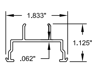
11 FIXED PANEL SUPPORT
