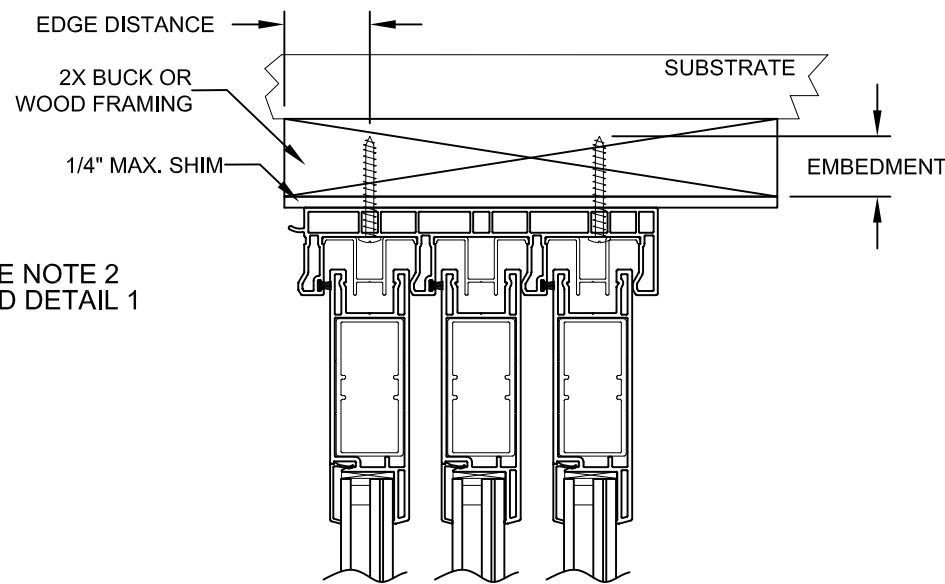
3 VERTICAL CROSS SECTION 4 2X BUCK CONSTRUCTION (SEE NOTES 3 & 4)
