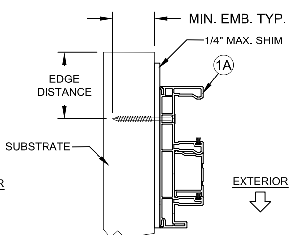
⑩ HORIZONTAL CROSS SECTION ③ MASONRY CONSTRUCTION (SEE NOTES 4 & 5)
