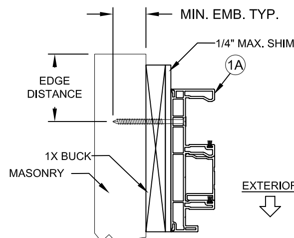
⑨ HORIZONTAL CROSS SECTION ③ 1X BUCK CONSTRUCTION (SEE NOTES 4 & 5)
