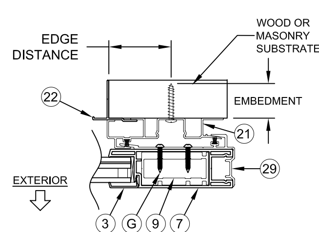
⑧ HORIZONTAL CROSS SECTION ③ HOOKSTRIP (SEE NOTE 5)
