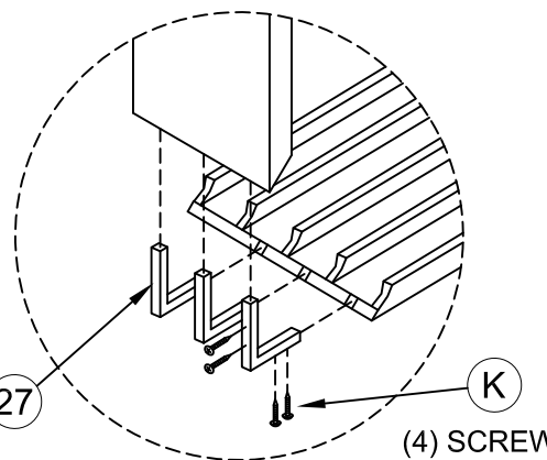
CORNER DETAIL
