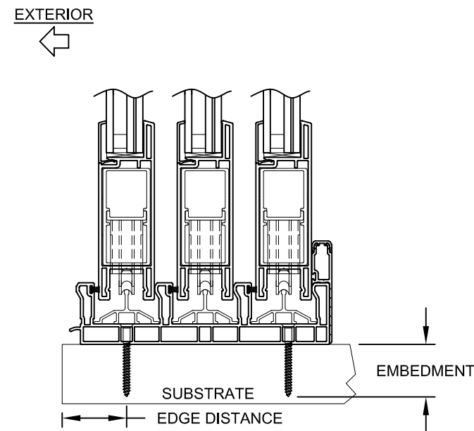
4 VERTICAL CROSS SECTION 4 MASONRY CONSTRUCTION (SEE NOTES 3 & 4)
