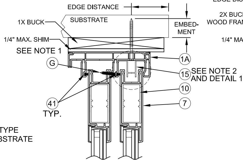
1 VERTICAL CROSS SECTION 4 1X BUCK CONSTRUCTION (SEE NOTES 3 & 4)
