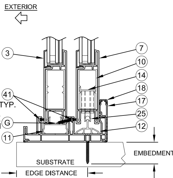
2 VERTICAL CROSS SECTION 4 MASONRY CONSTRUCTION (SEE NOTES 3 & 4)
