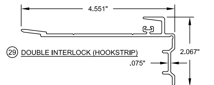
21 HOOKSTRIP
