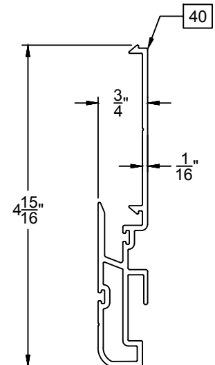
P-Hook - 2063 6063-T6
