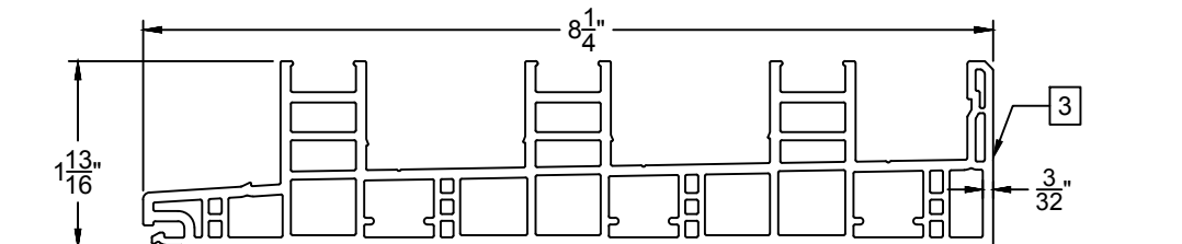
3-Track Sill - 6163
