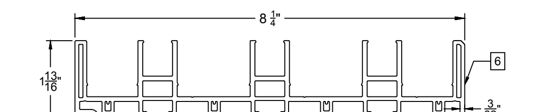
3-Track Head/Jamb - 6162
