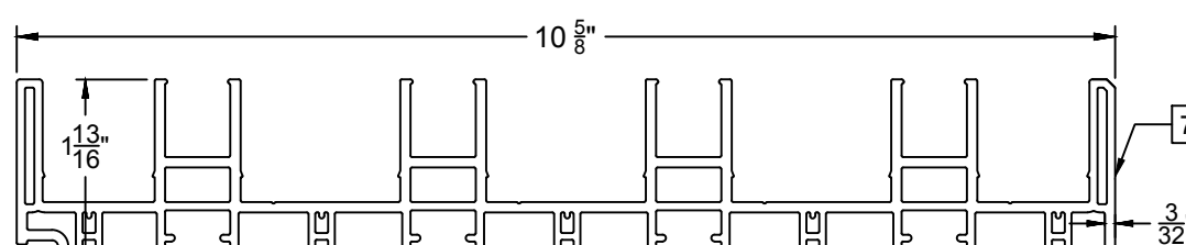
4-Track Head/Jamb - 6164
