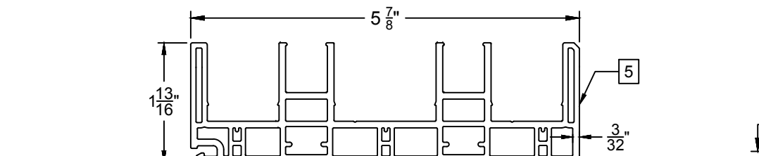
2-Track Head/Jamb - 6160
