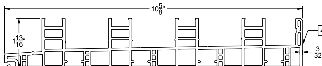
4-Track Sill - 6165
