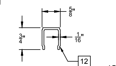
Track Filler - 6175
