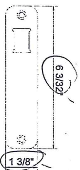
33 TOP/BOTTOM BAR KEEPER STAINLESS STEEL
