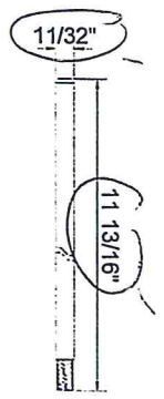
28 FLUSH BOLT BAR STAINLESS STEEL
