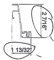
11 OUTSWING SILL-(B) ALUMINUM
