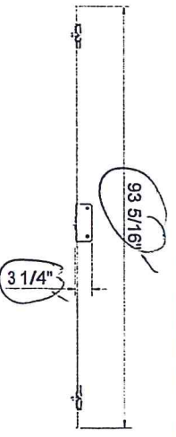
30 MULTI-POINT LOCKING SYSTEM STAINLESS STEEL, STEEL
