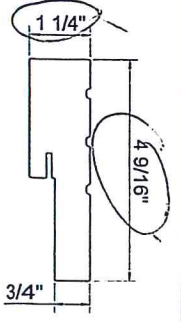
1 HEAD FRAME & JAMB FOAM PVC CO-EX.
