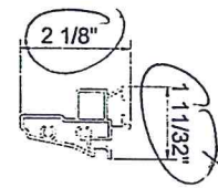
17 REINFORCEMENT (B) ALUMINUM
