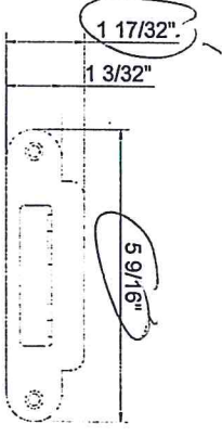
34 SLAB MULTI-POINT LOCK KEEPER STAINLESS STEEL
