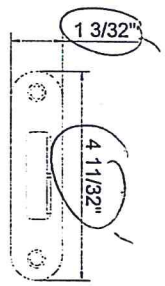
32 HEAVY HOOK KEEPER STAINLESS STEEL
