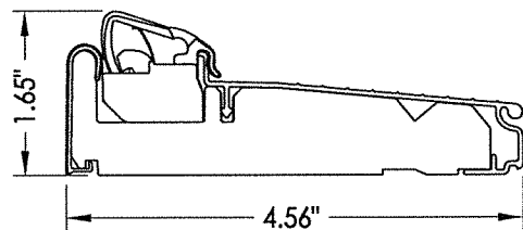
7 INSWING ARTICULATING THRESHOLD ZAC4565FN MAX. DESIGN PRESSURE = +40/-45 PSF
