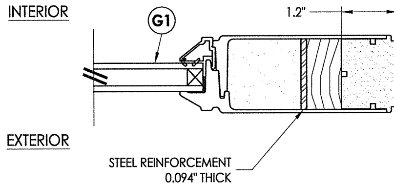
1 5 HORIZONTAL CROSS SECTION
