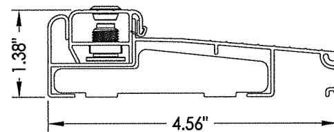
3 INSWING ADJUSTABLE THRESHOLD ZAILAA4565 MAX. DESIGN PRESSURE = +40/-45 PSF
