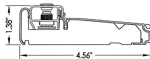
4 INSWING ADJUSTABLE THRESHOLD ZAI4565RDS MAX. DESIGN PRESSURE = +40/-45 PSF
