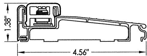
1 INSWING ADJUSTABLE THRESHOLD ZAIL4565 MAX. DESIGN PRESSURE = +40/-45 PSF
