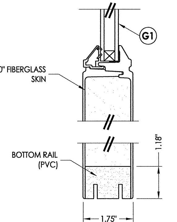
2 5 VERTICAL CROSS SECTION
