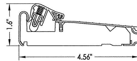
9 INSWING ARTICULATING THRESHOLD ZACAA4565FN MAX. DESIGN PRESSURE = +40/-45 PSF
