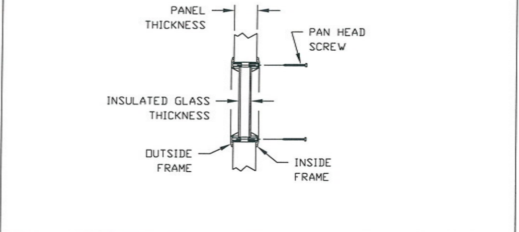
STANDARD ASSEMBLY DETAILS DRAWING 104801-B
