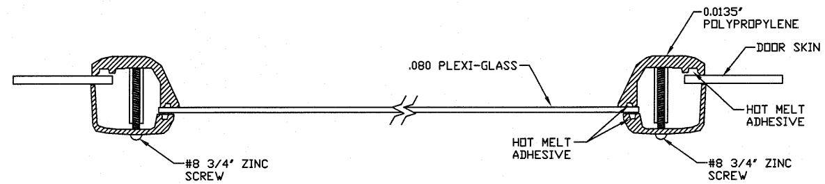
SECTION B-B 24' X 12' WINDOW DETAIL N.T.S.
