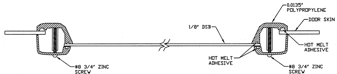
SECTION C-C 24' X 6' WINDOW DETAIL N.T.S.
