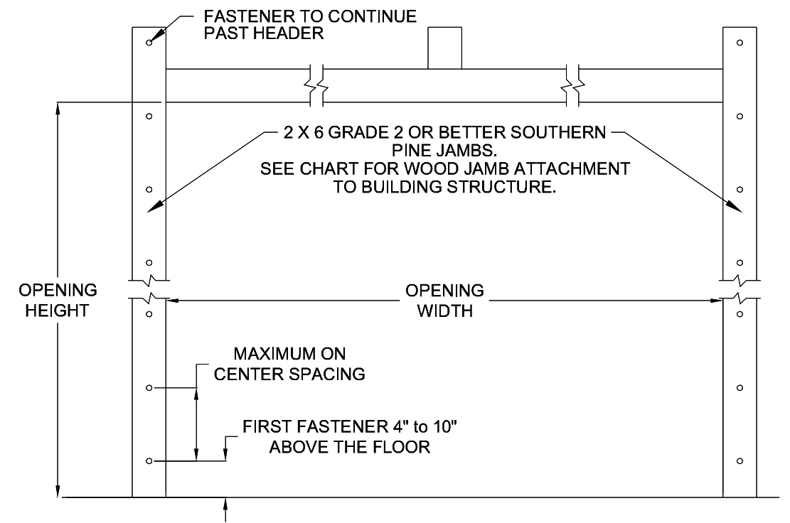
SCREW LOCATION - COMMERCIAL LITES NOTE: 10 SCREWS USED.
