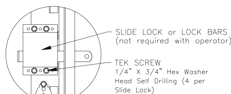
DETAIL G
