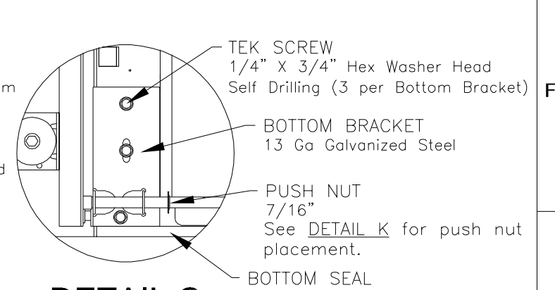
DETAIL C
