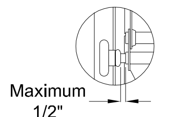
DETAIL K
