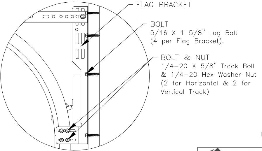
DETAIL H
