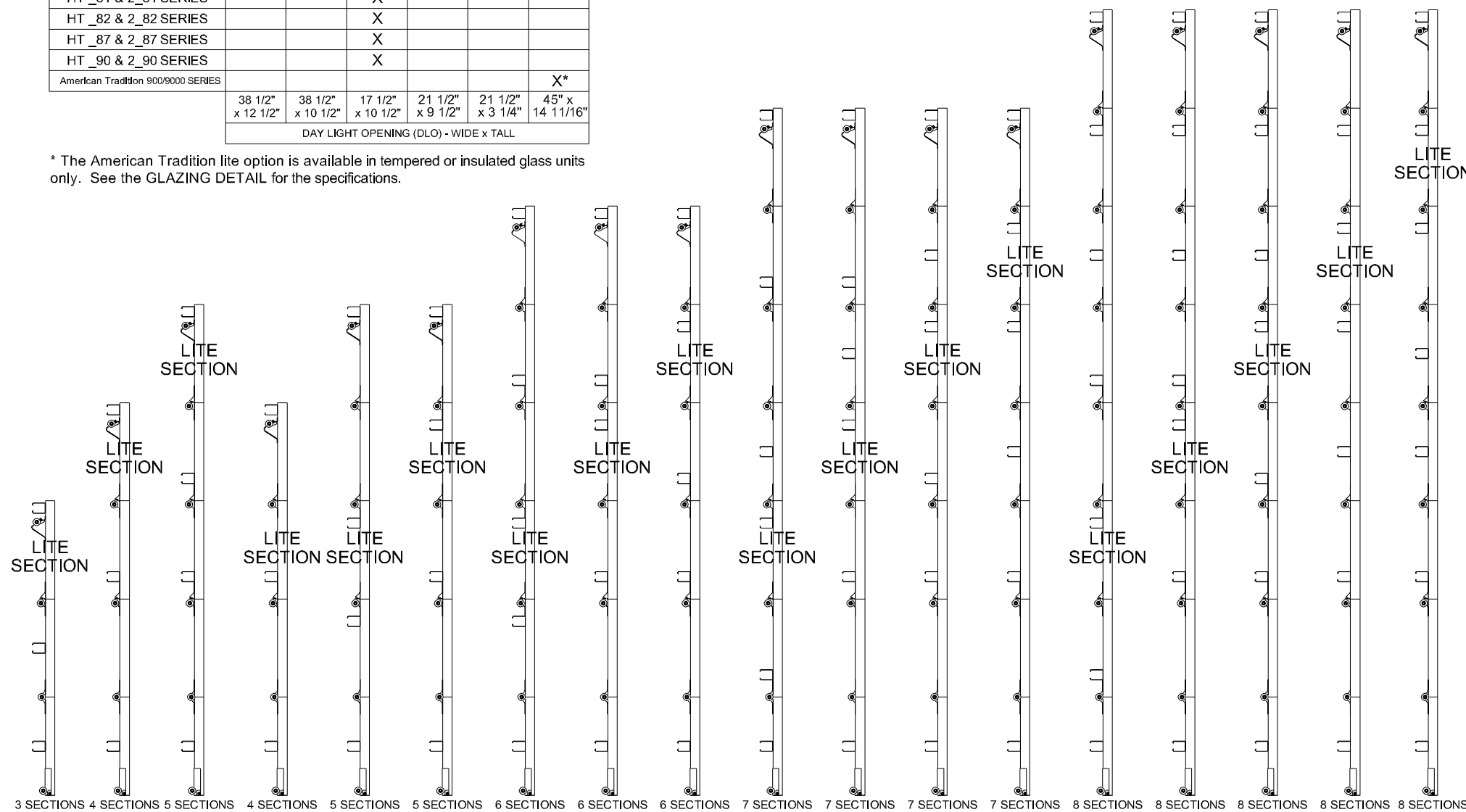
WITH LITE SECTION AT TOP WITH LITE SECTION ANYWHERE EXCEPT THE TOP AND BOTTOM SECTION STRUT CONFIGURATION
