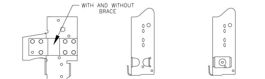
DETAIL D
