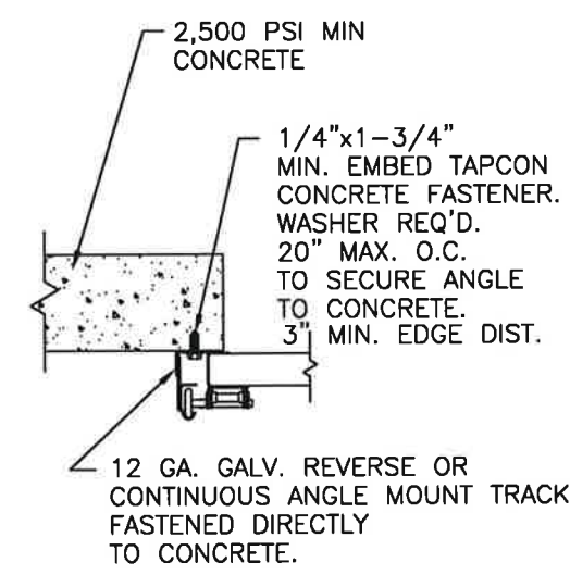
SECTION 3-3
