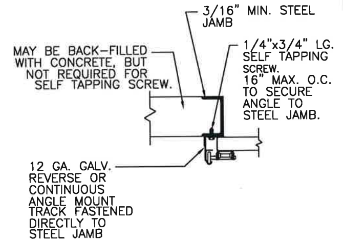
SECTION 3-3
