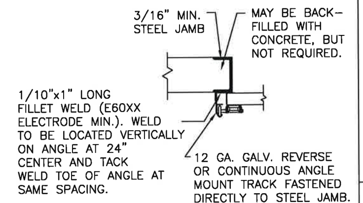
SECTION 3-3
