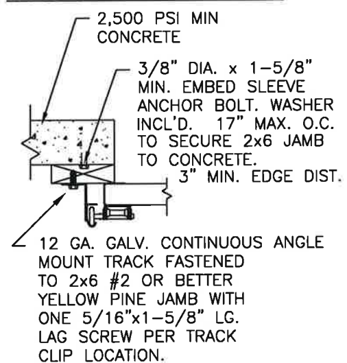
SECTION 3-3
