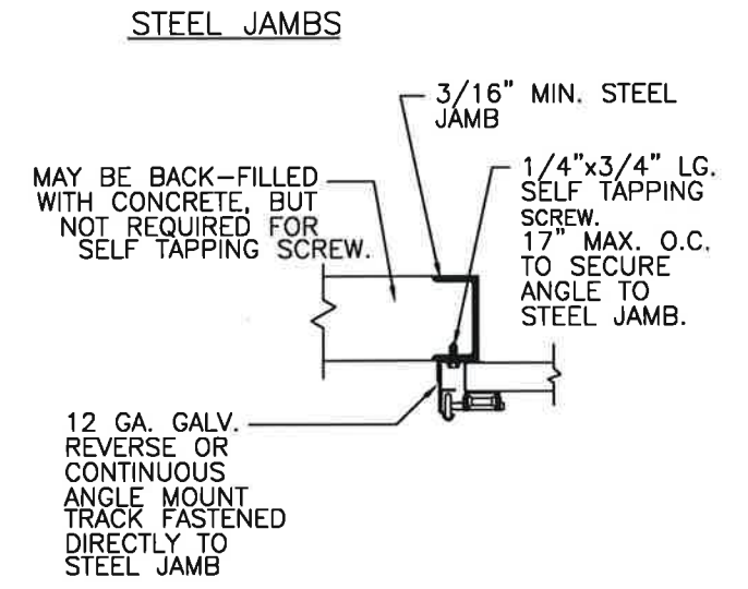
SECTION 3-3
