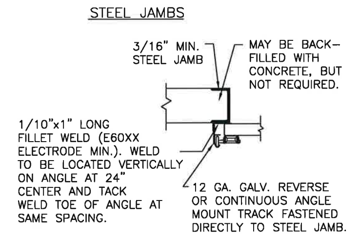
SECTION 3-3
