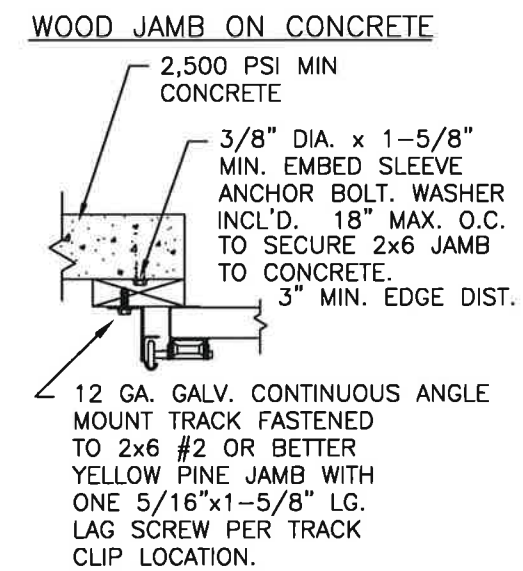
SECTION 3-3
