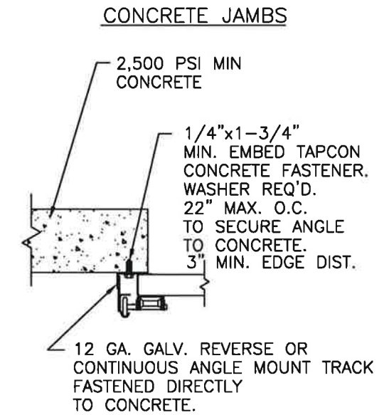
SECTION 3-3
