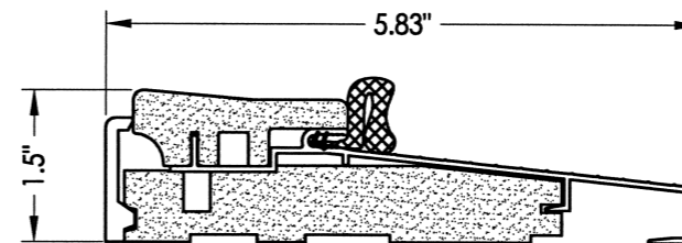
14 OUTSWING THRESHOLD
