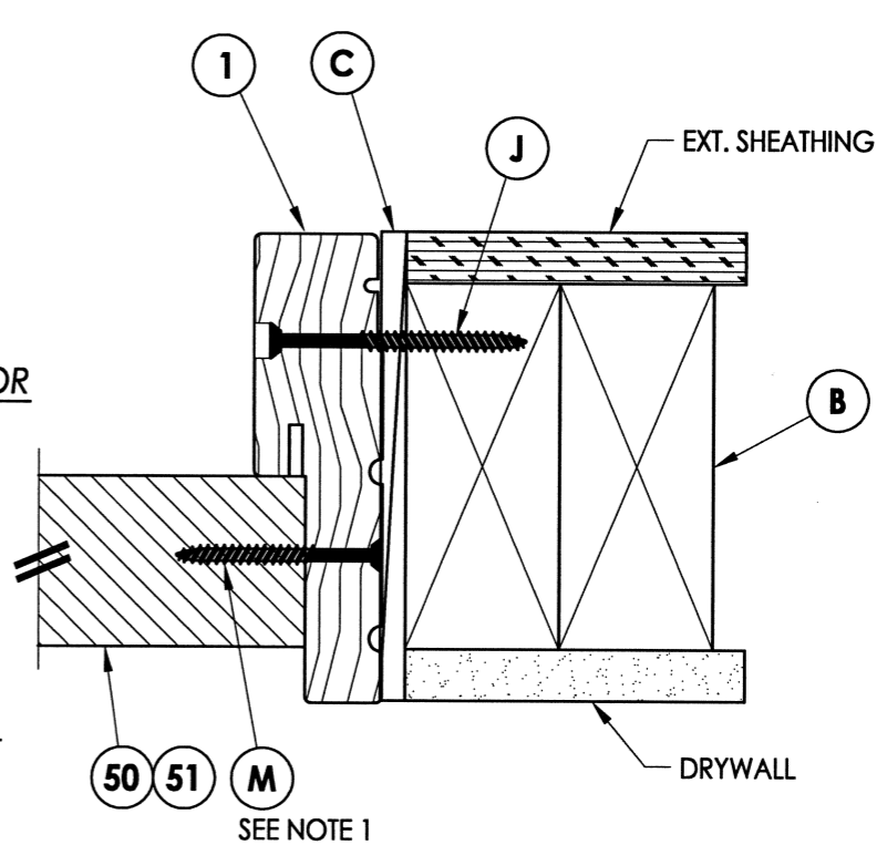
3 HORIZONTAL CROSS SECTION 7 Inswing shown - Outswing also approved
